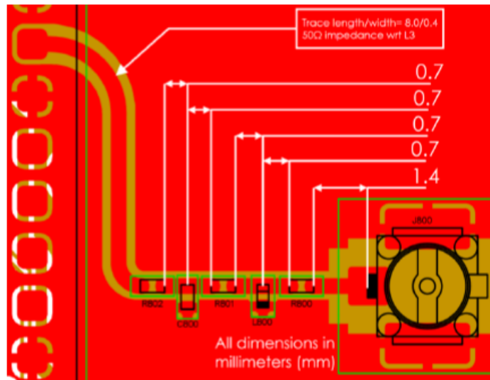
Figure 2: PCB Design Guideline
