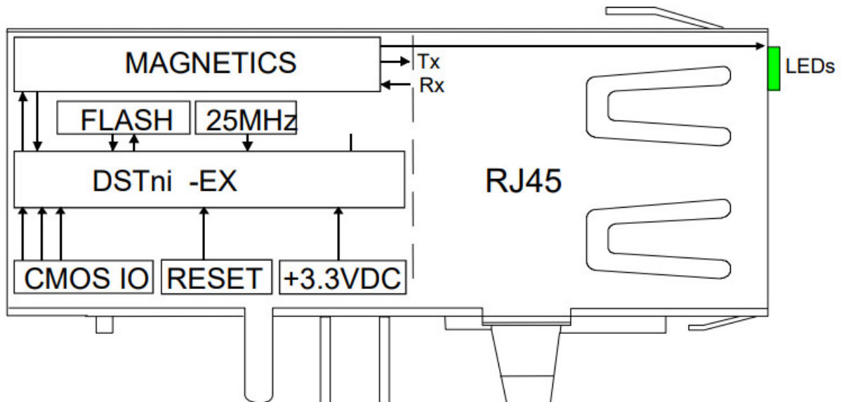
Figure 2-1 Side View of the XPort
