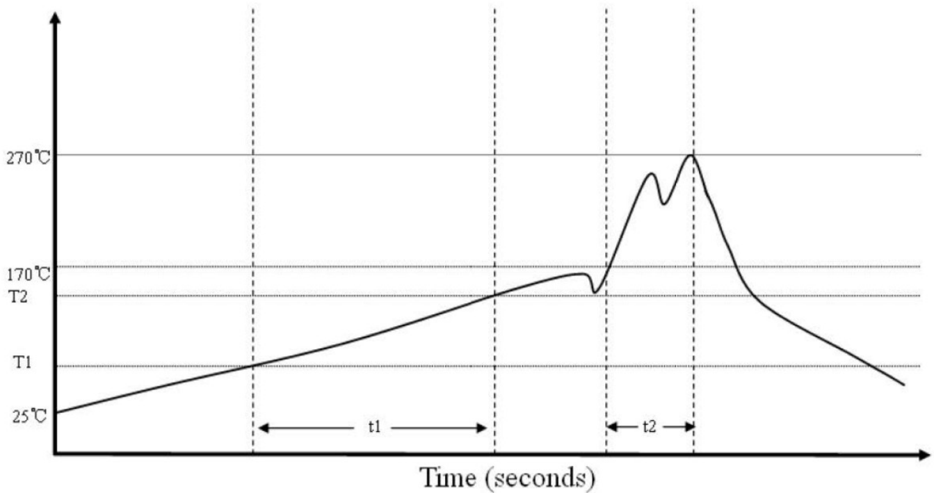
Figure 2-8 [WS-A] Wave Soldering – Recommended Profile
