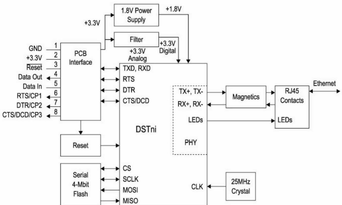
Figure 2-2 XPort Block Diagram
