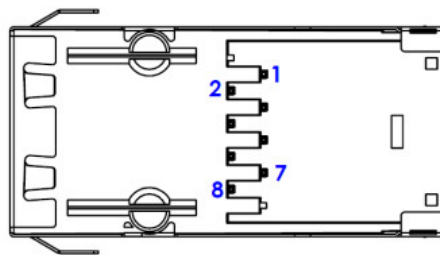
Figure 2-5 Bottom View
