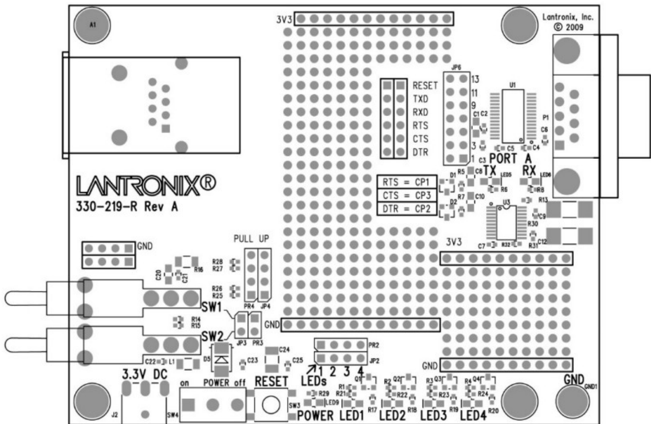
Figure 3-1 XPort Demo Board Layout
