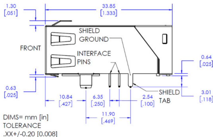
Figure 2-6 Side View
