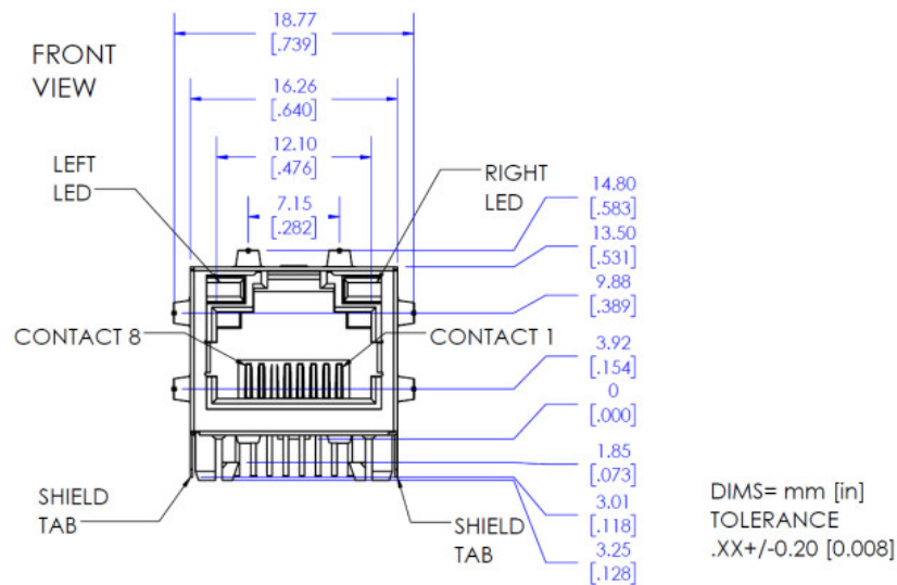
Figure 2-4 Front View
