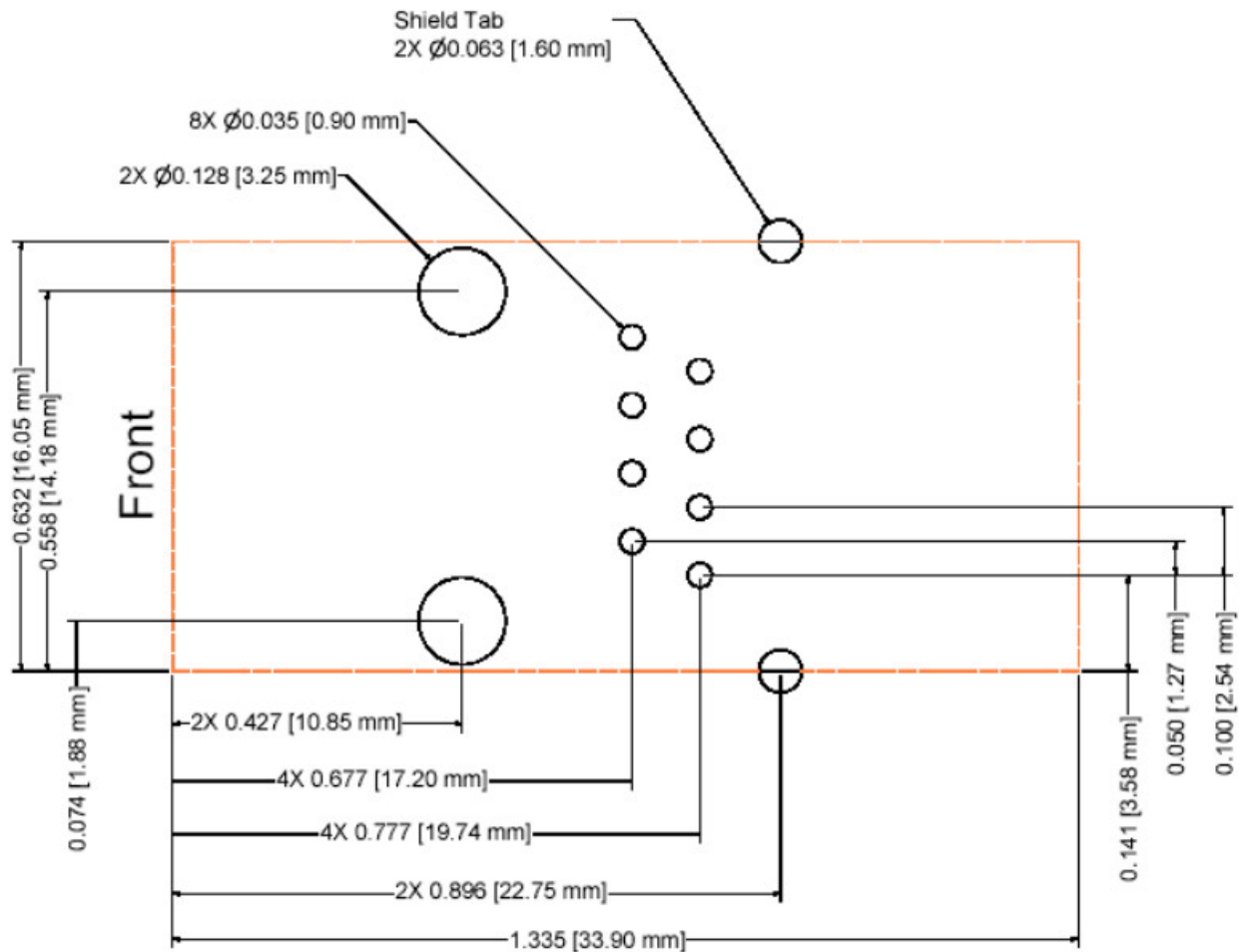
Figure 2-7 PCB Layout
