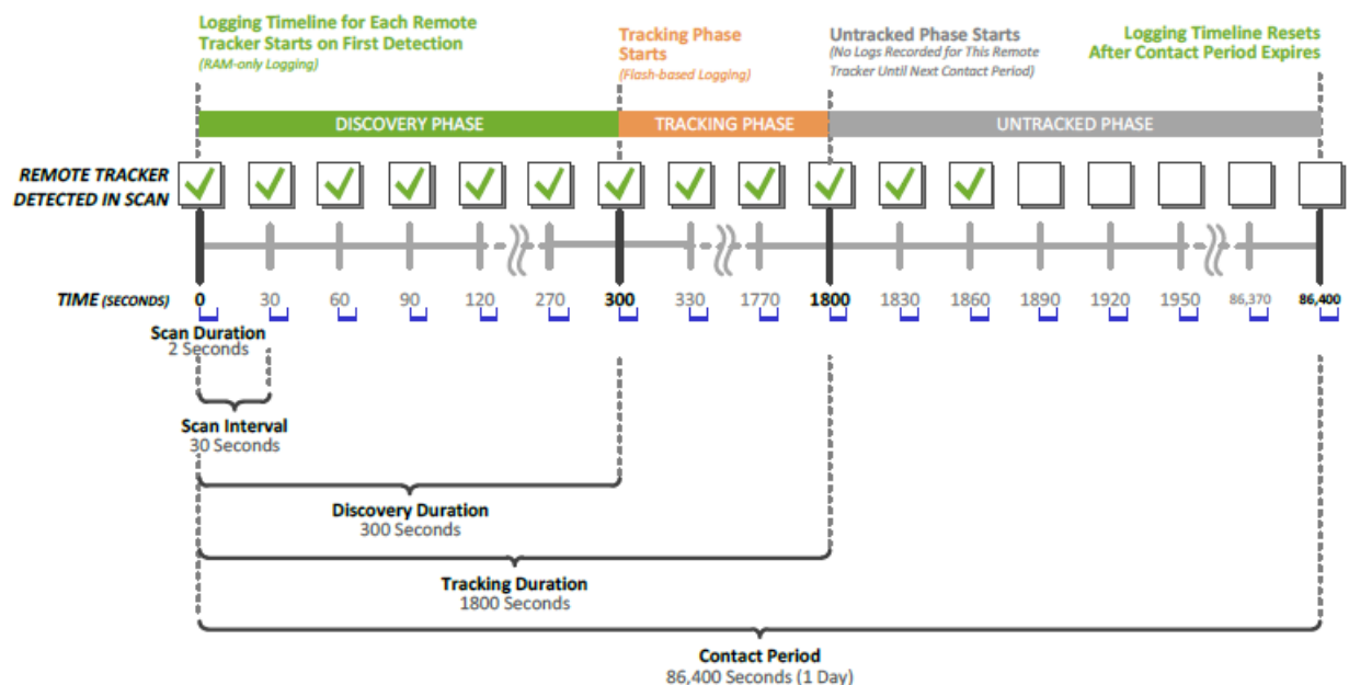
Figure 5 - Data logging timeline
