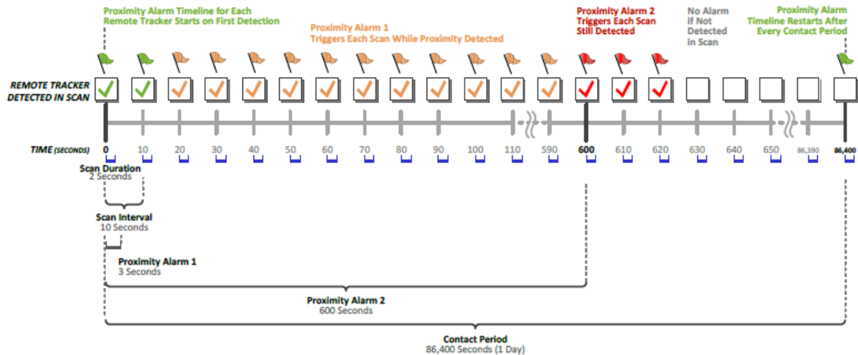
Figure 4 - Proximity alarm timeline
