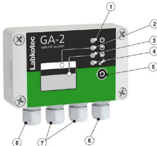
Figure 2. GA-2 Grease Alarm –features
