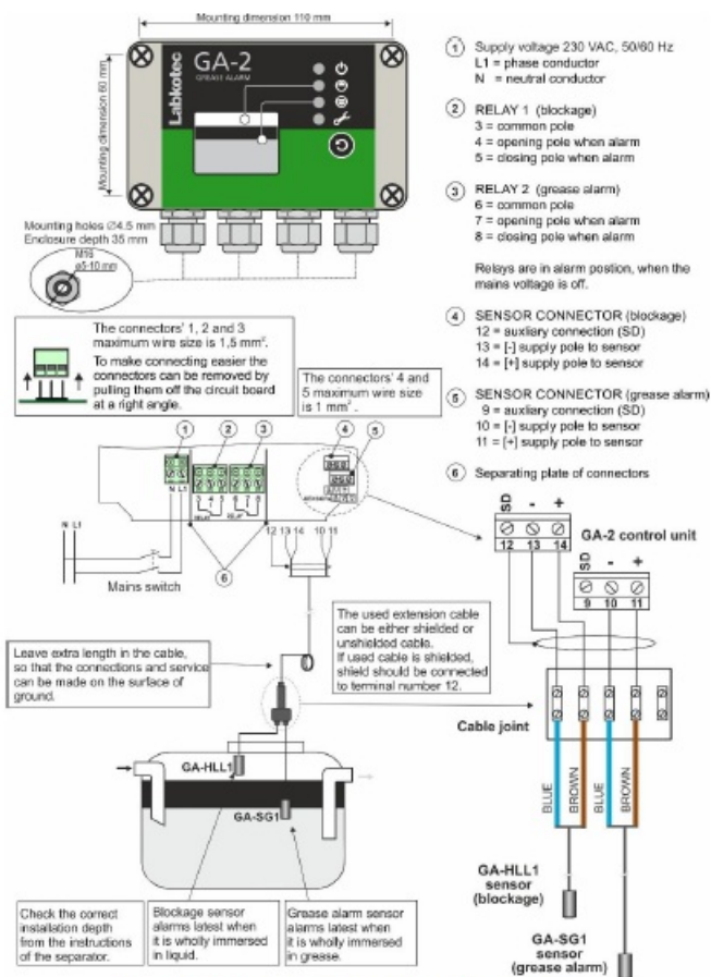
Figure 3. Installation of GA-2 Grease Alarm device.
