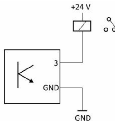
Figure 5 . Example connection
