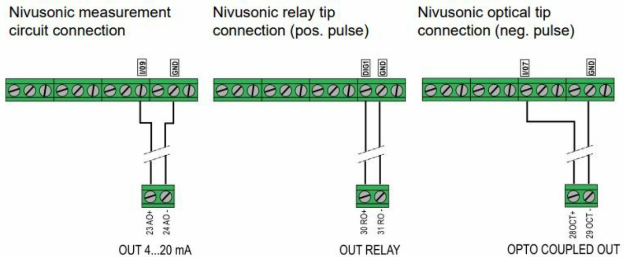
Figure 13 . Labcom 221 GPS – Nivusonic CO 100 S; Connection
