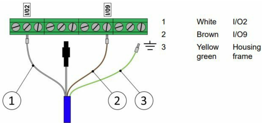
Figure 12 . Labcom 221 GPS – DMU-08 and L64 sensors; Connection
