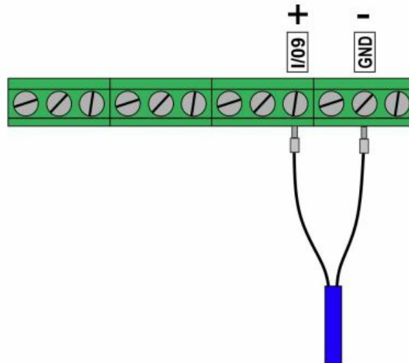
Figure 4 . Example connection
