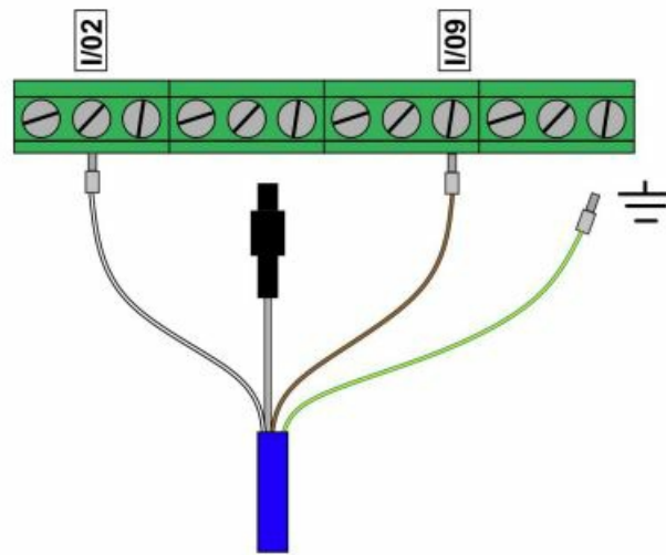
Figure 3 . Example connection
