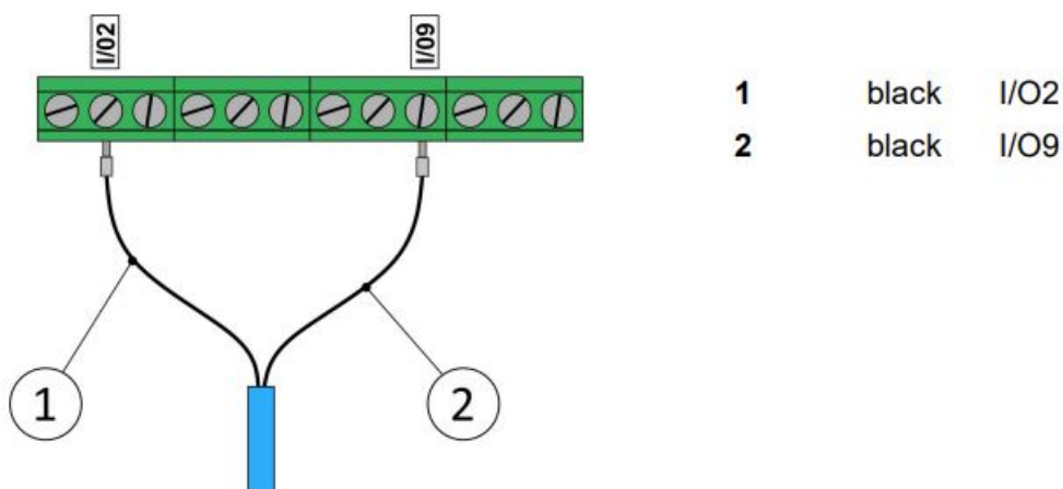
Figure 7 . Labcom 221 GPS - idOil-LIQ sensor; Connection
