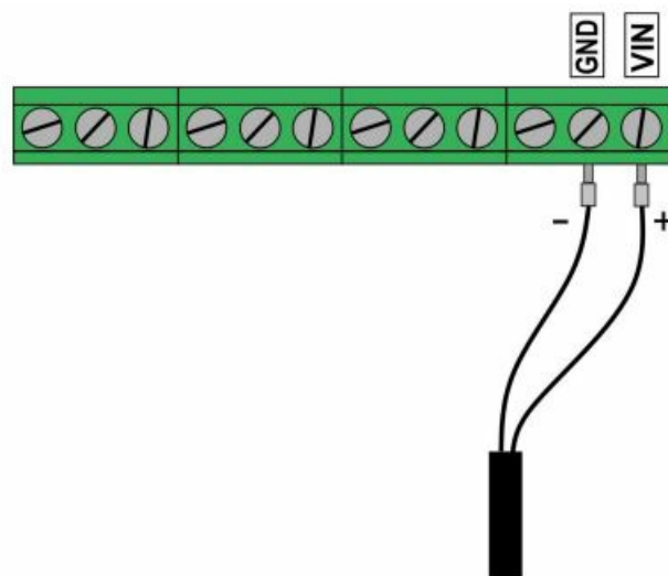
Figure 14 . External voltage supply; Connection
