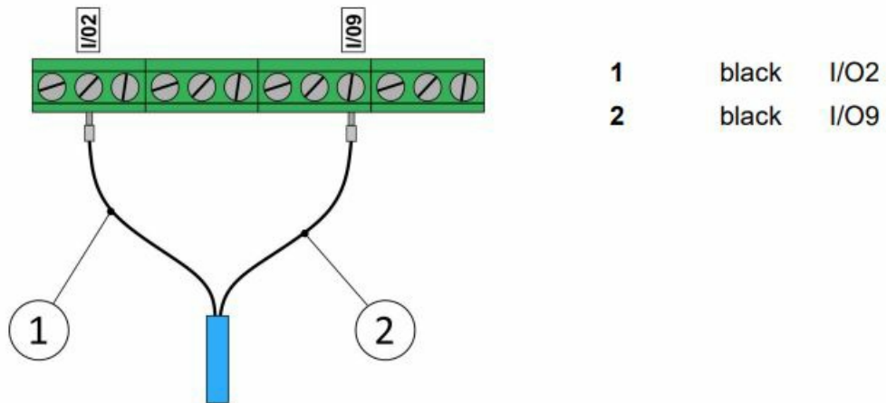
Figure 9 . Labcom 221 GPS - GA-SG1 sensor; Connection
