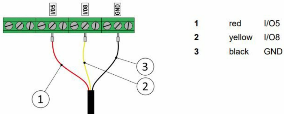
Figure 11 . Labcom 221 GPS – 1-wire temperature sensor; Connection
