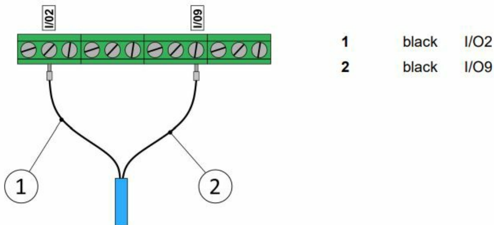
Figure 8 . Labcom 221 GPS – idOil-SLU sensor; Connection
