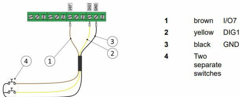
Figure 6 . Example connections
