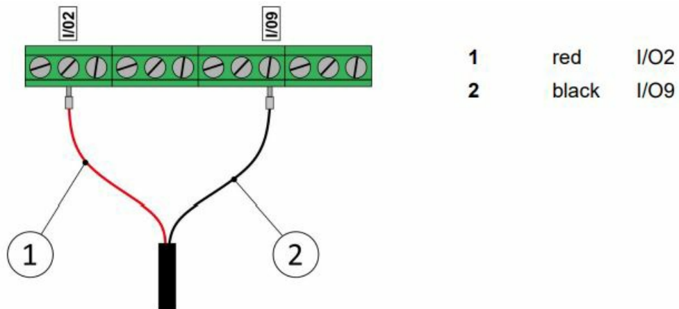
Figure 10 . Labcom 221 GPS - SGE25 sensor; Connection
