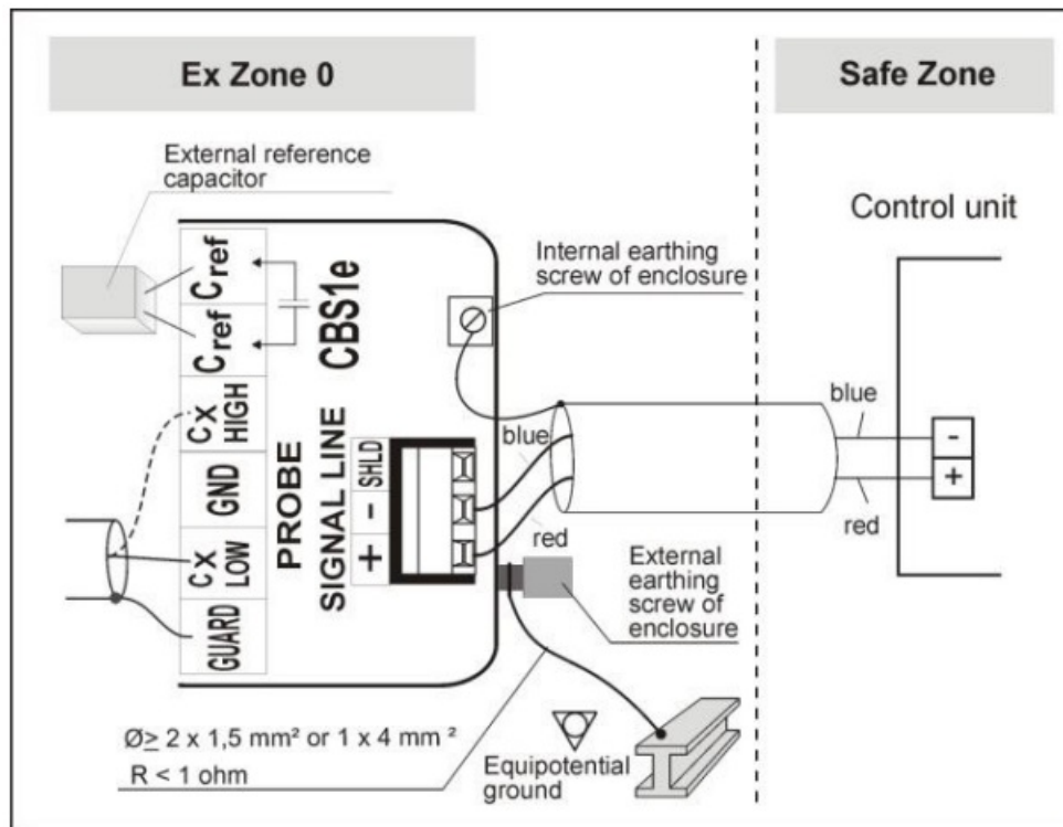
Fig. 3. Connection example
