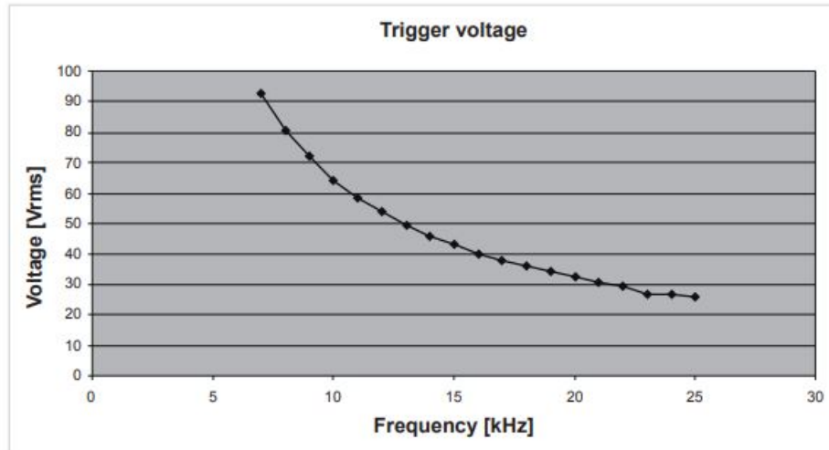
Fig 11.4: VHF Protection Frequency Sensitivity
