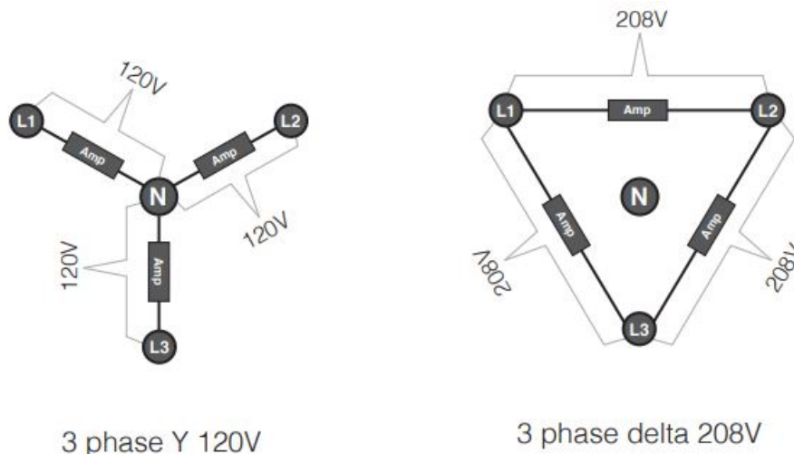
Figure 6:4: Three phase delta configuration
