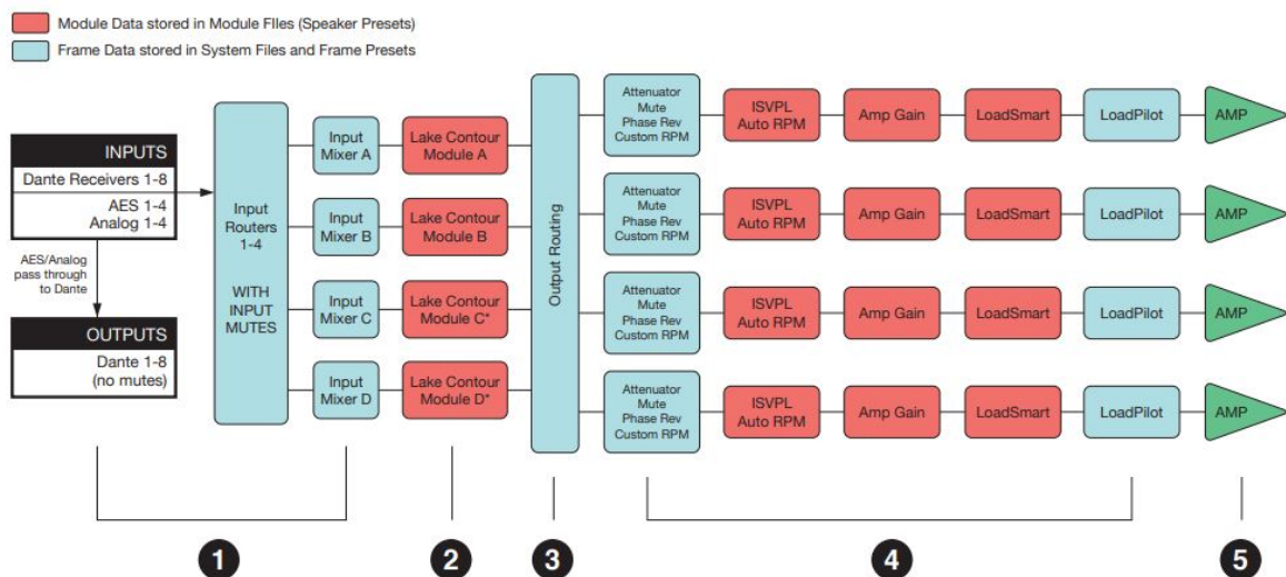
Figure 8.1: D Series Lake Signal Flow Diagram
