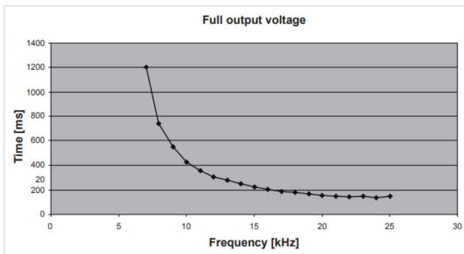
Fig 11.5: VHF Protection Attack Time Variations
