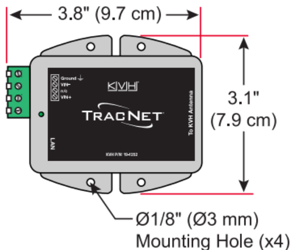
Figure 12: PoE Injector Dimensions
