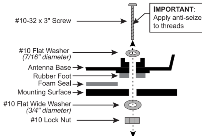
Figure 11: Mounting Hardware
