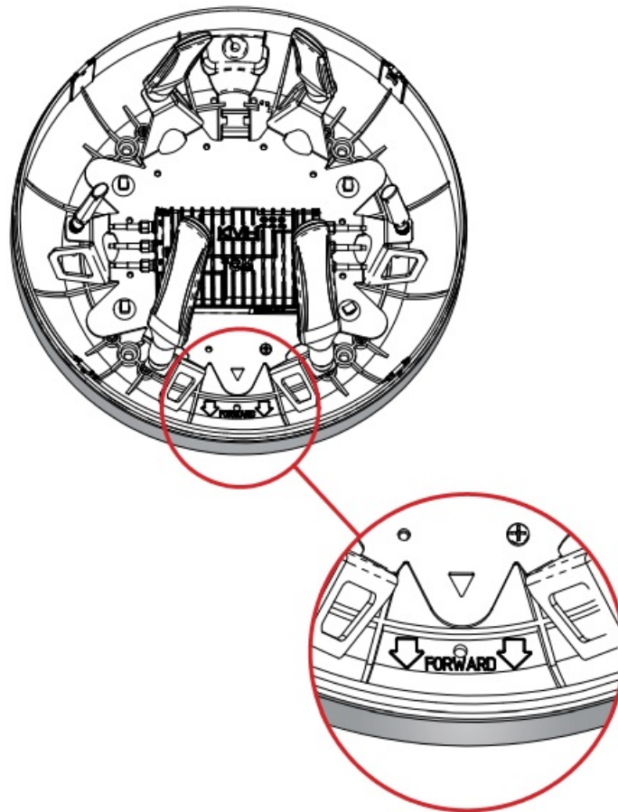
Figure 10: Forward Arrow in Antenna Baseplate
