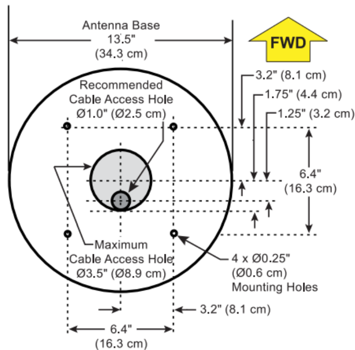
Figure 5: Antenna Mounting Holes Layout
