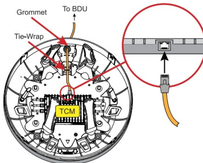
Figure 9: Connecting the Ethernet Cable
