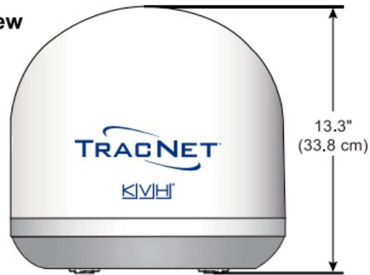
Figure 2: Antenna Dimensions
