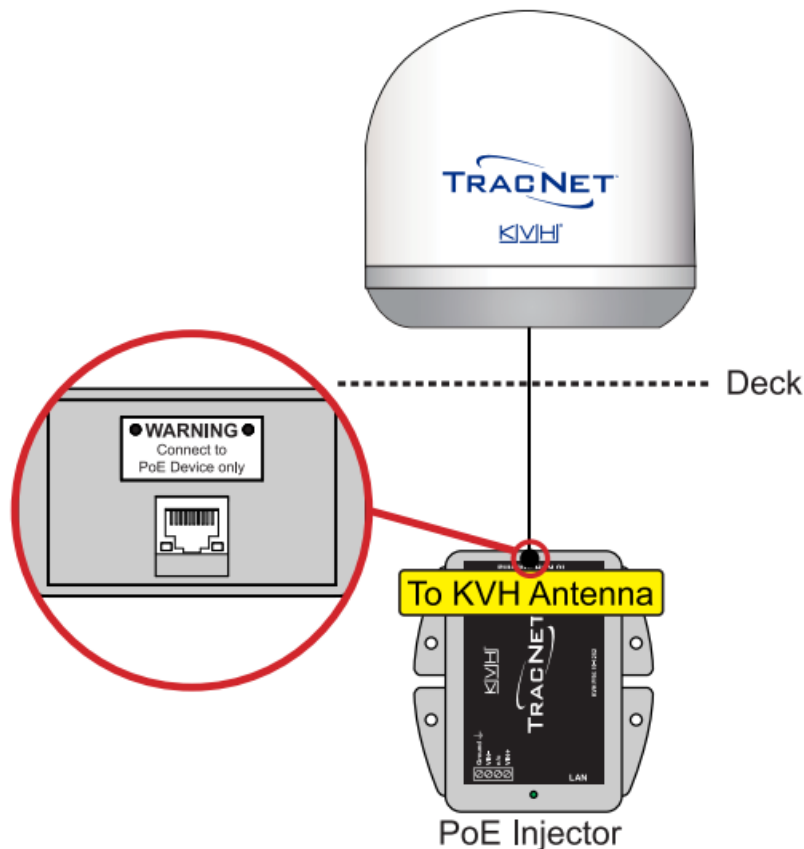
Figure 13: PoE Injector Antenna Connection
