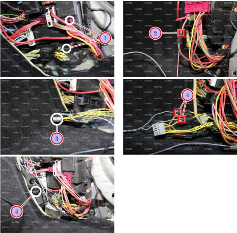
Figure 5: Connection cable set
