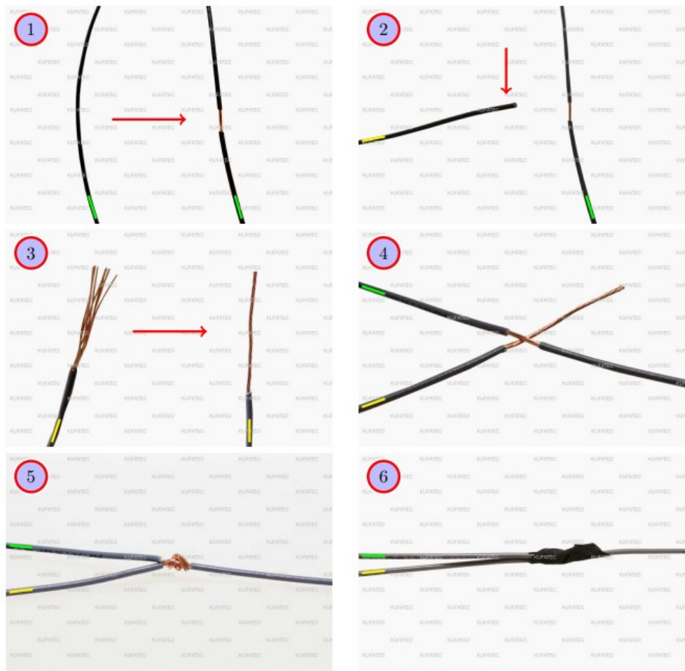
Figure 1: How to connect a cable to another
