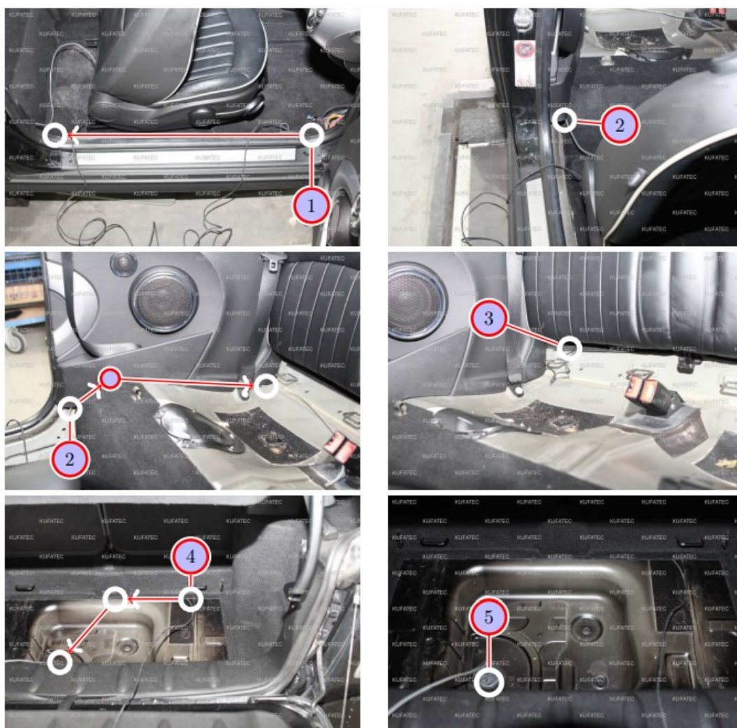
Figure 7: Cable routing to the sound generator
