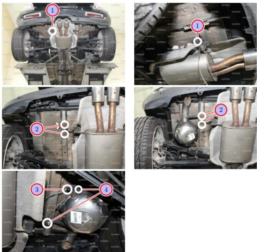
Figure 8: Installation / connection sound generator
