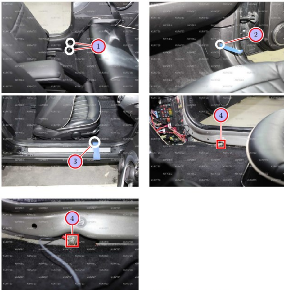
Figure 4: Removing sill trim / connection ground
