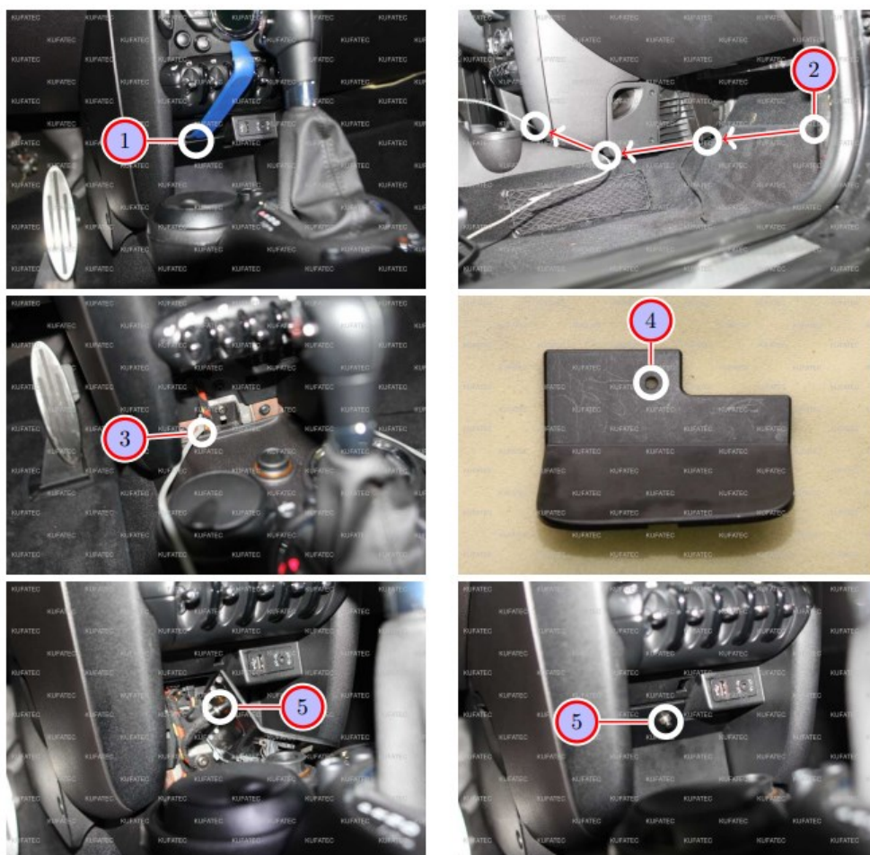
Figure 9: Installation pushbutton
