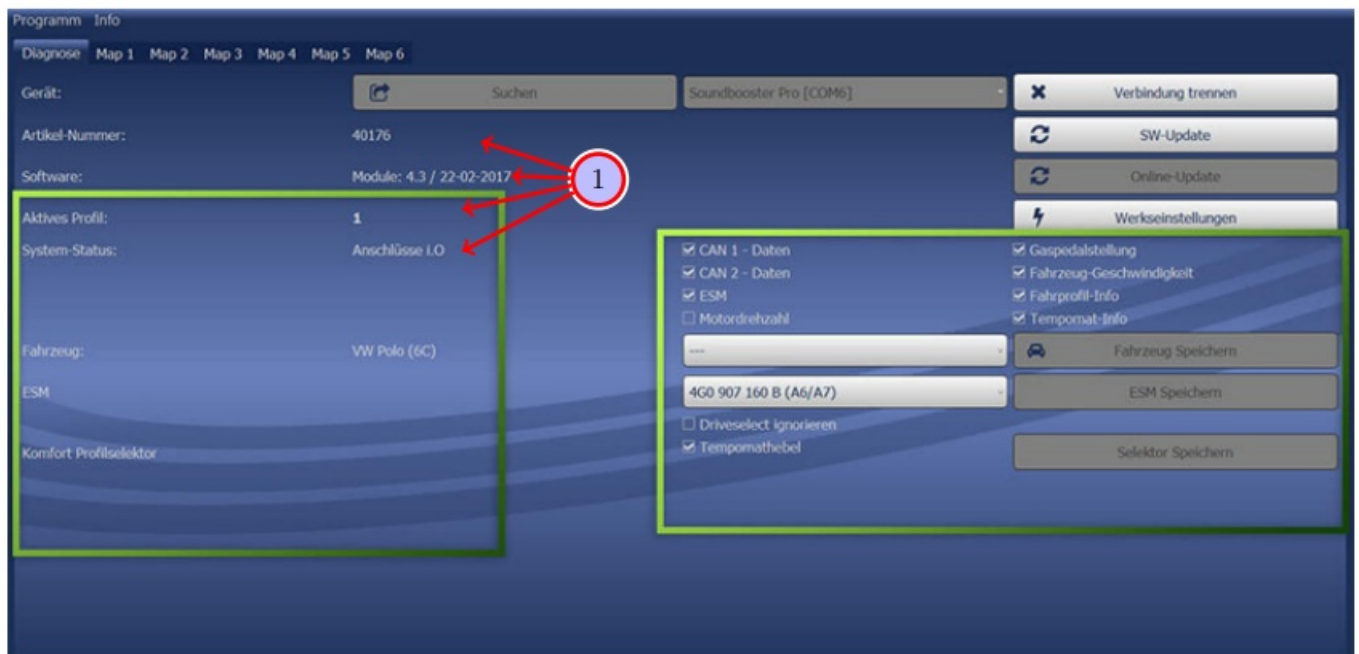
Figure 9: Software
