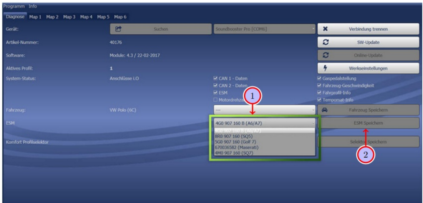
Figure 11: Software
