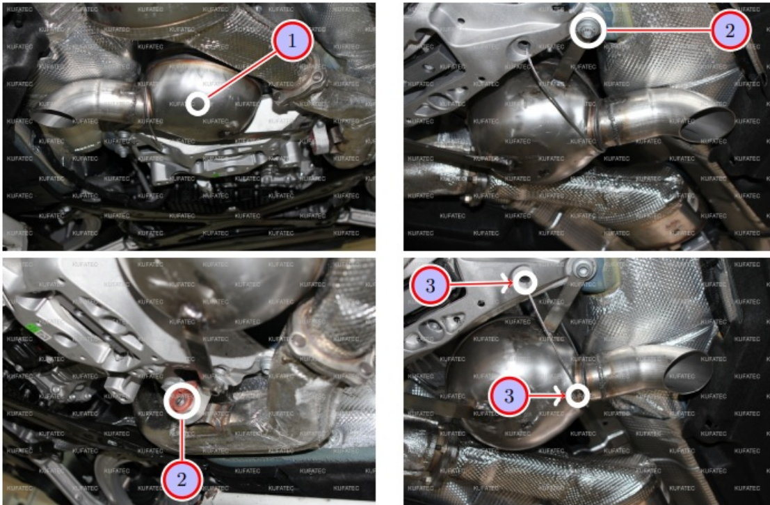
Figure 8: Installation sound generator
