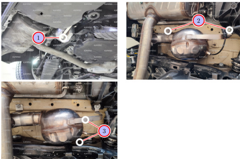
Figure 6: Installation sound generator, Version 1 - 4 cylinders 2.0 Liter
