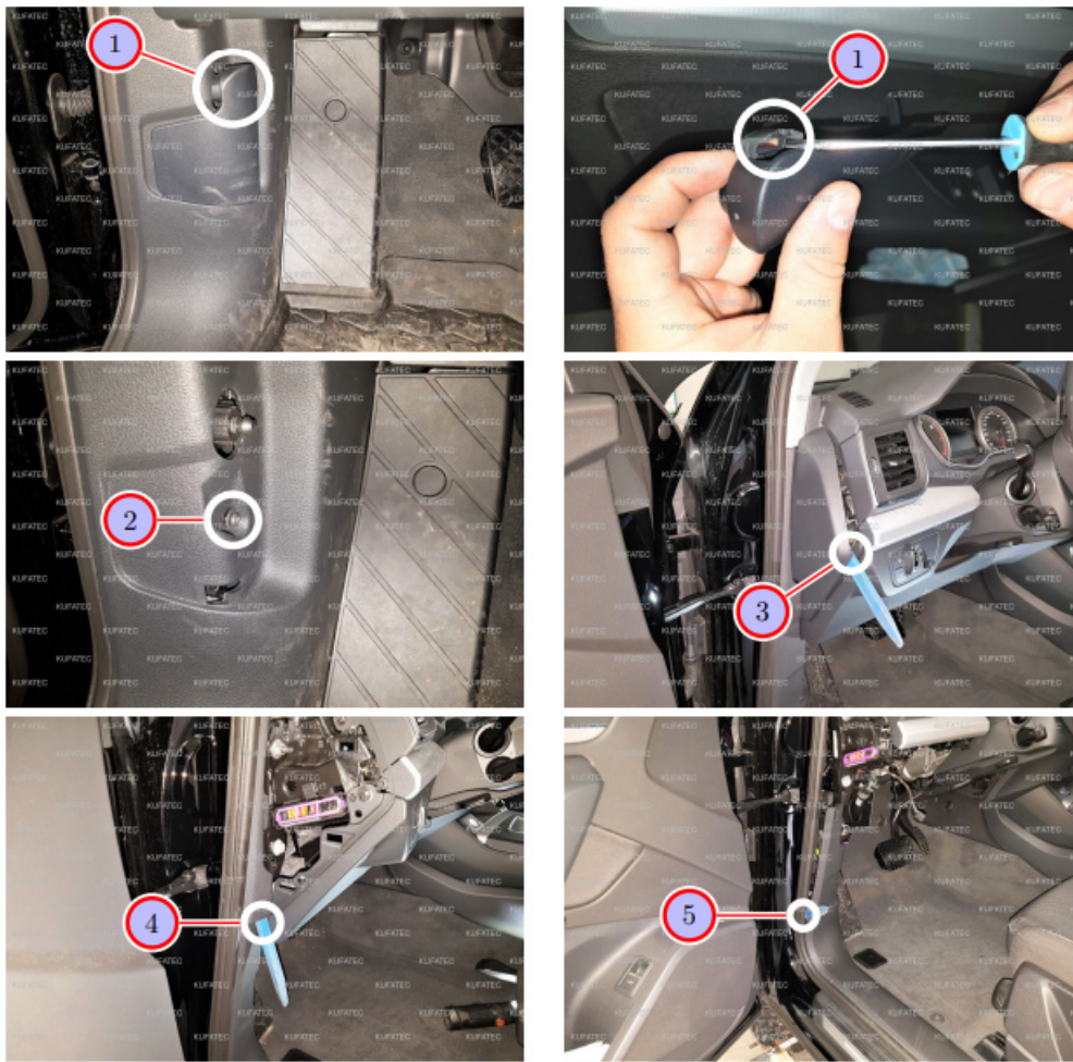
Figure 4: Disassembly trim parts on driver's side
