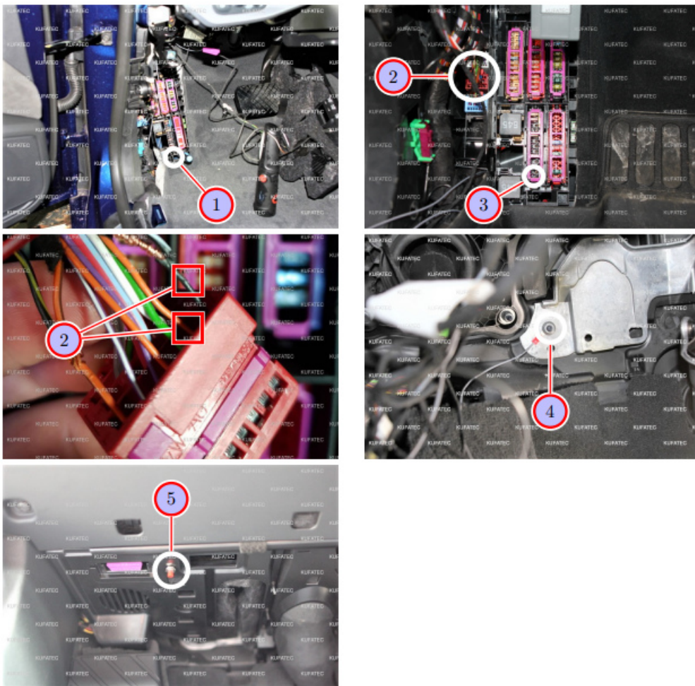
Figure 8: Connection CAN high + low / ground / push button
