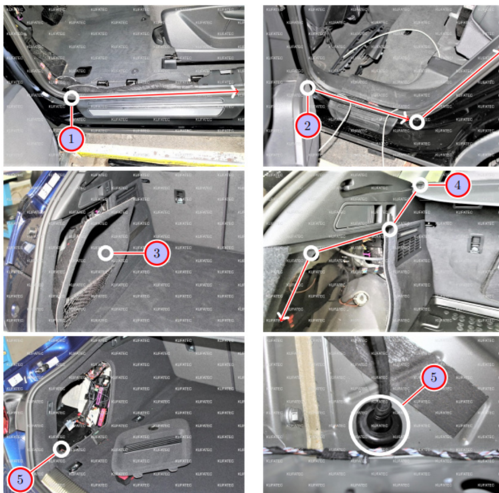
Figure 9: Cable routing to the sound generator
