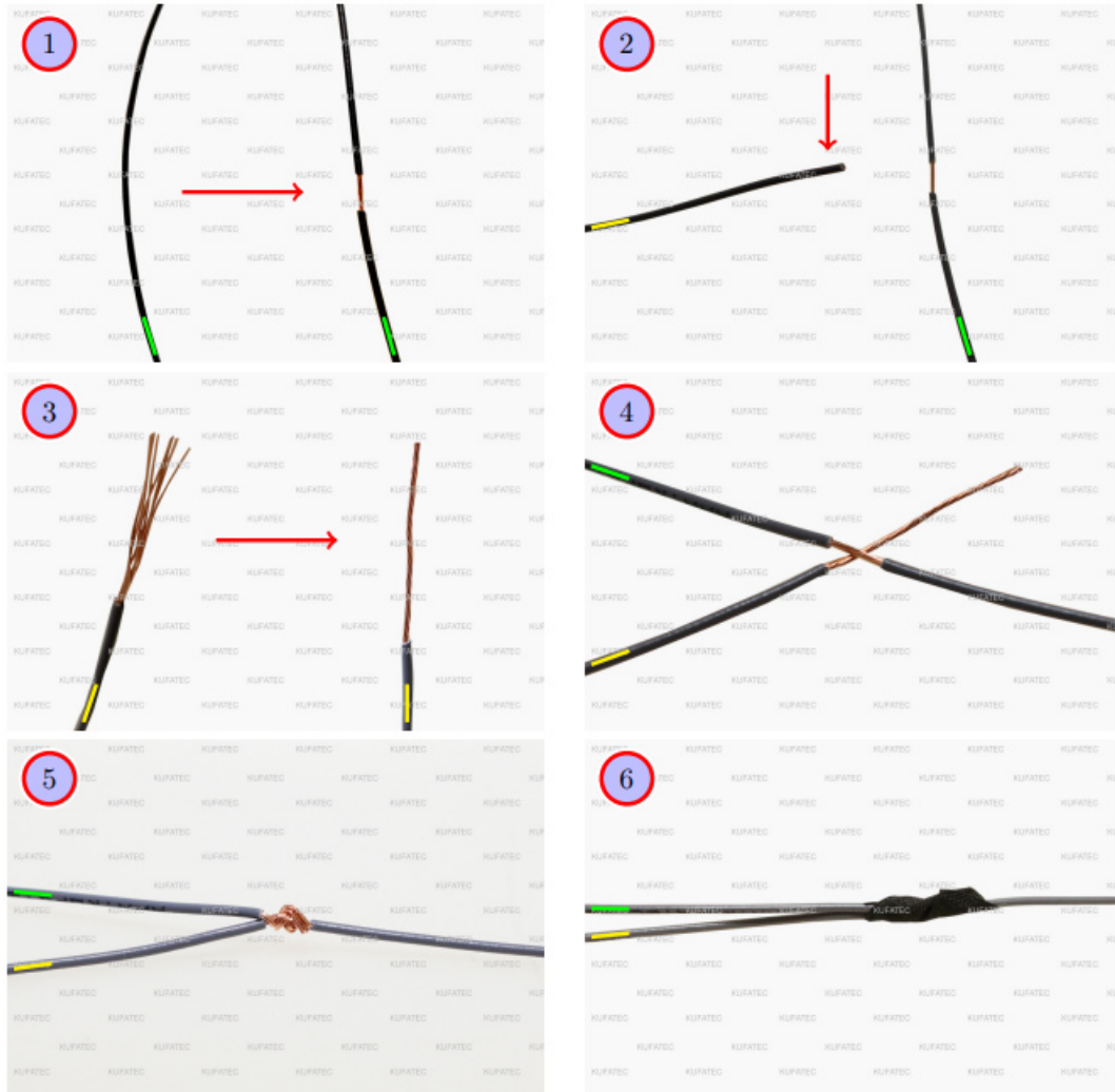
Figure 1: How to connect a cable to another
