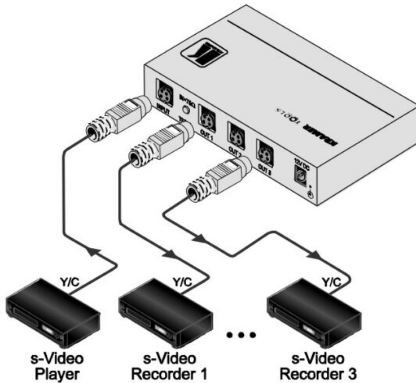
Figure 5: Connecting the VM-3SN s-Video Distributor
