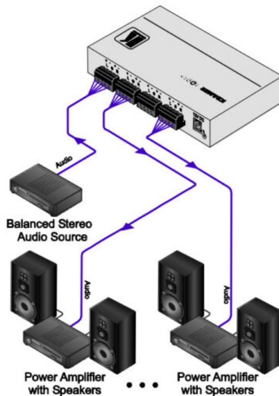
Figure 4: Connecting the VM-3AN Audio Distributor
