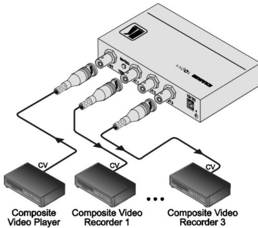
Figure 6: Connecting the VM-3VN Video Distributor
