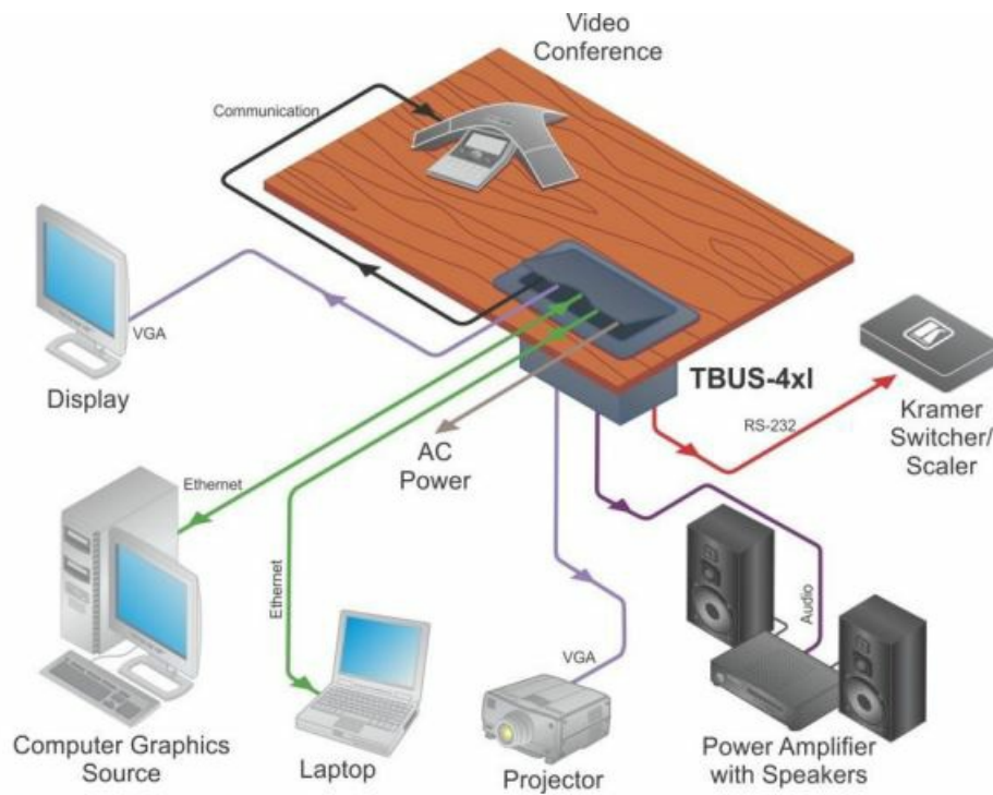
Figure 6: TBUS-4xl Boardroom Installation
