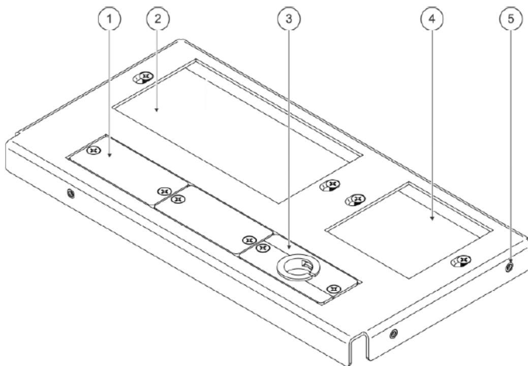
Figure 2: TBUS-10xl Inner Frame (P/N: 80-000028)
