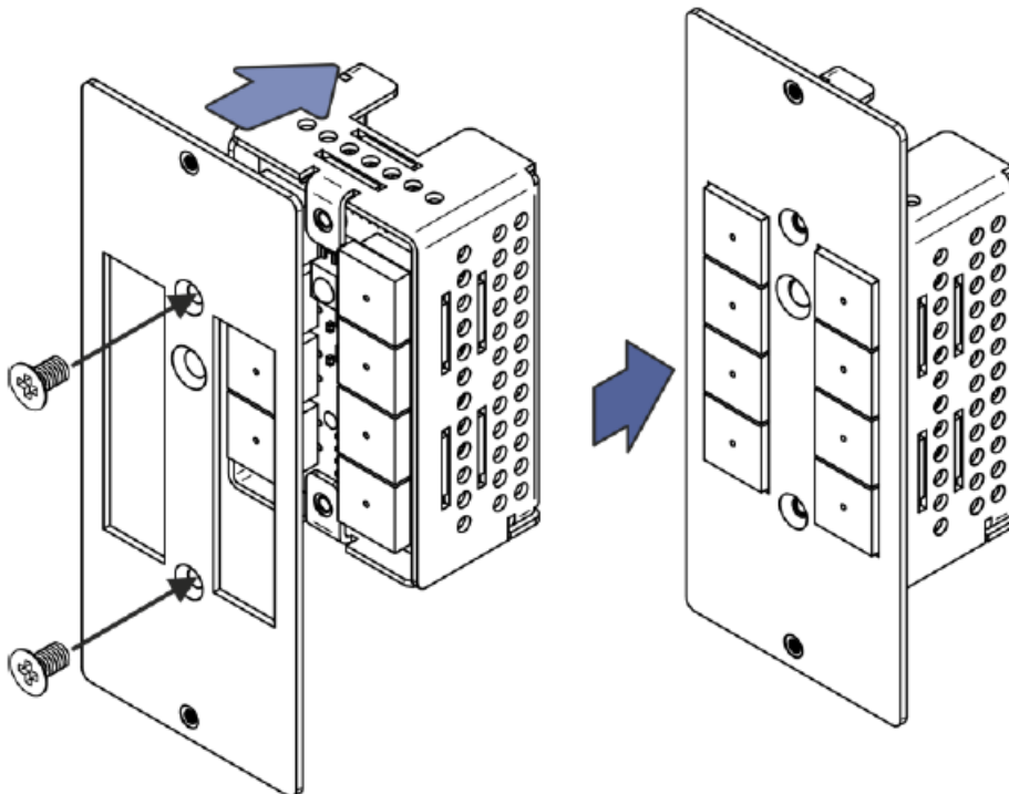
Figure 6: T-RC8IR Installation
