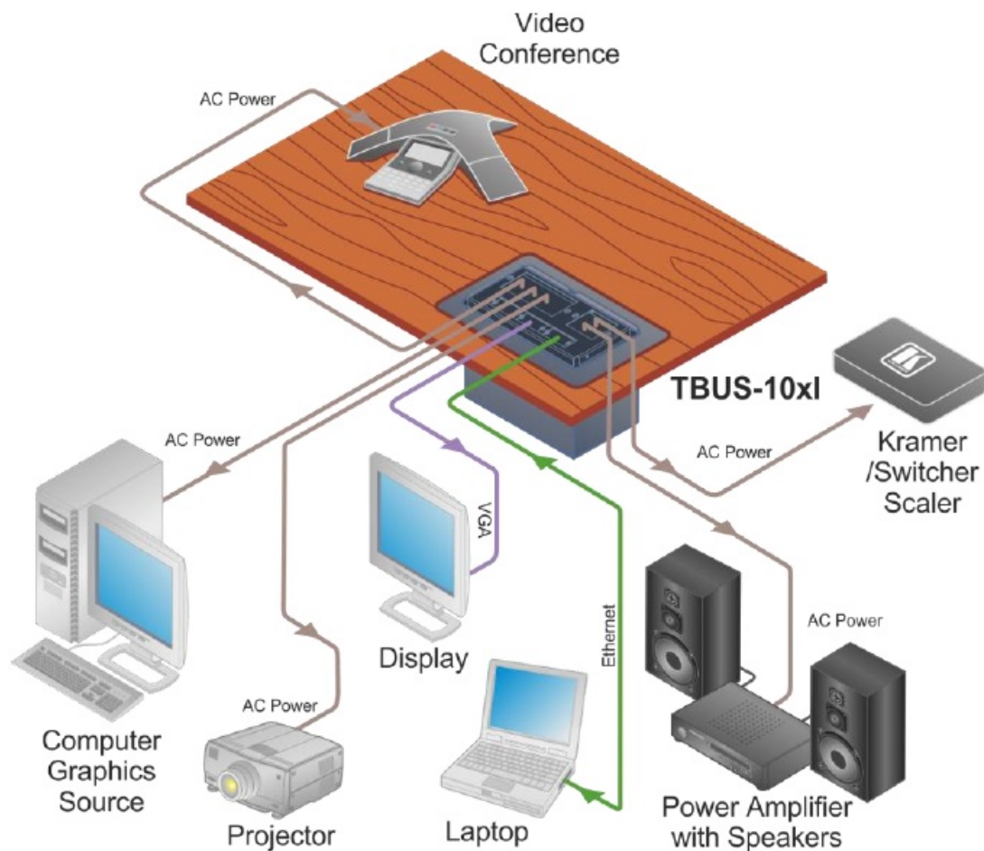
Figure 11: TBUS-10xl Boardroom Installation
