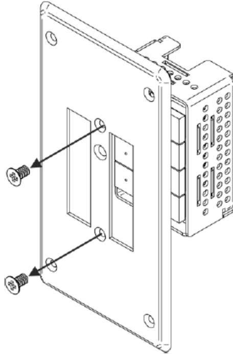
Figure 5: Removing the RC-8IR Faceplate
