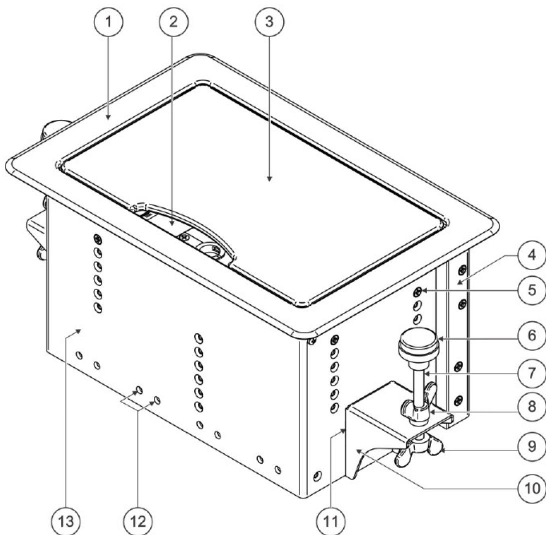
Figure 1: TBUS-10xl Enclosure Top View
