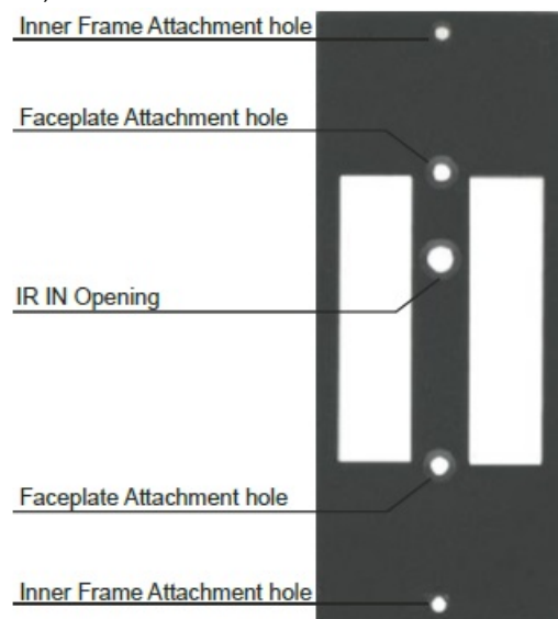
Figure 4: T-RC8IR (P/N: 80-000599)
