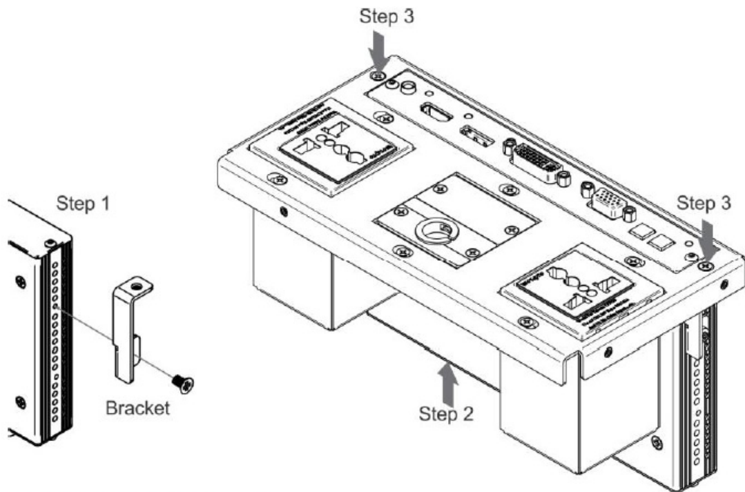
Figure 3: Installing the MegaTOOL
