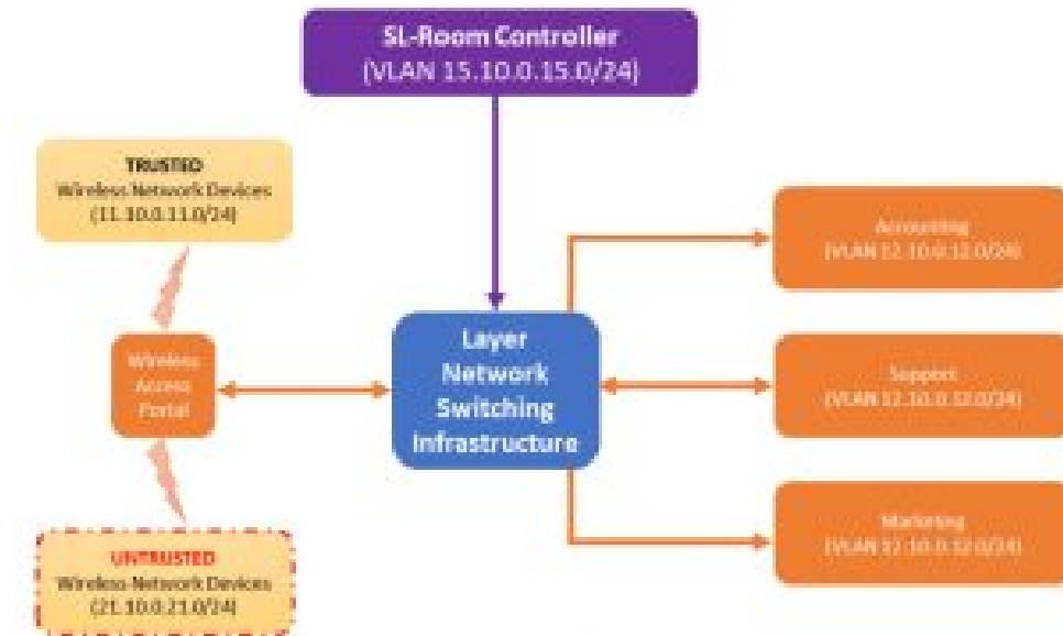
Figure 2: Segmented Network
