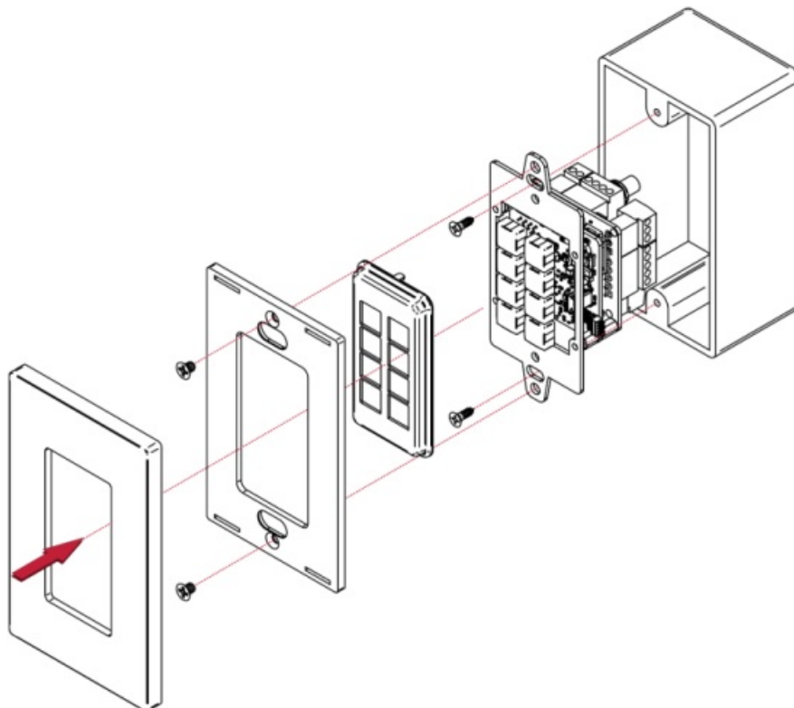
Figure 13: Installing the US-D Version
