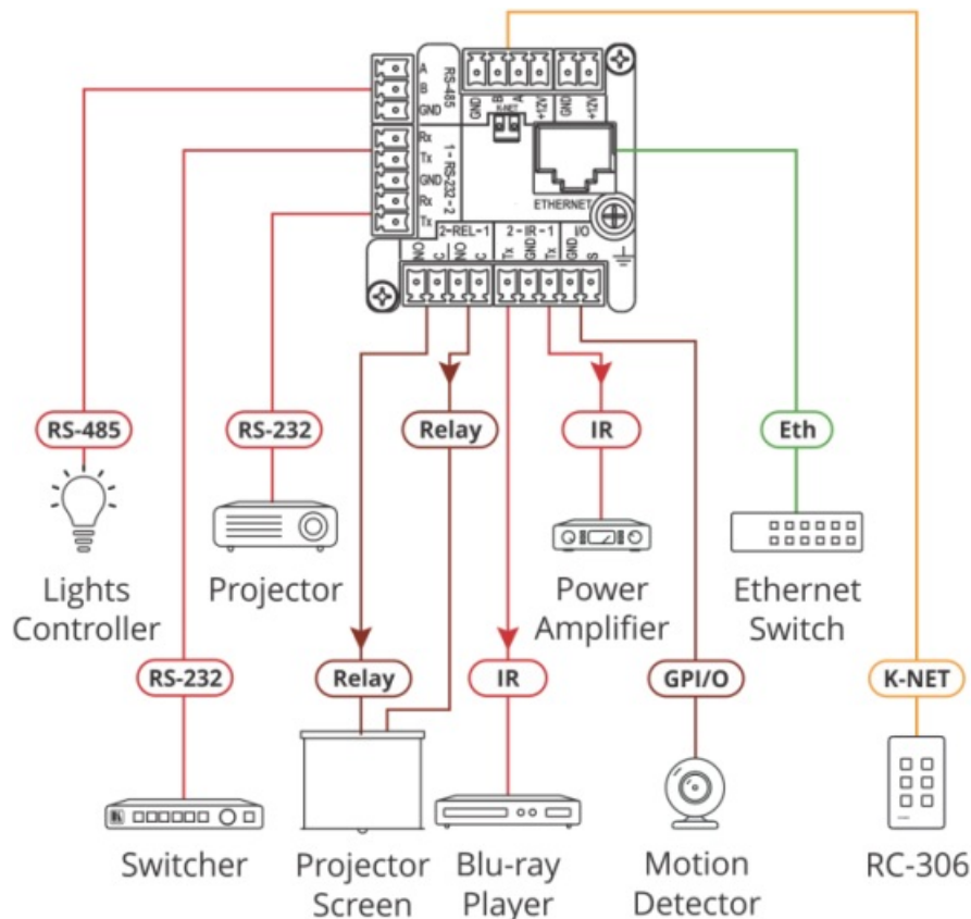
Figure 7: Connecting to the RC-308 Rear Panel
