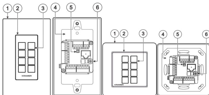
Figure 1: RC-308 and RC-208 Ethernet and K-NET Control Keypad Front Panel
