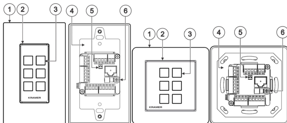
Figure 2: RC-306 and RC-206 Ethernet and K-NET Control Keypad Front Panel
