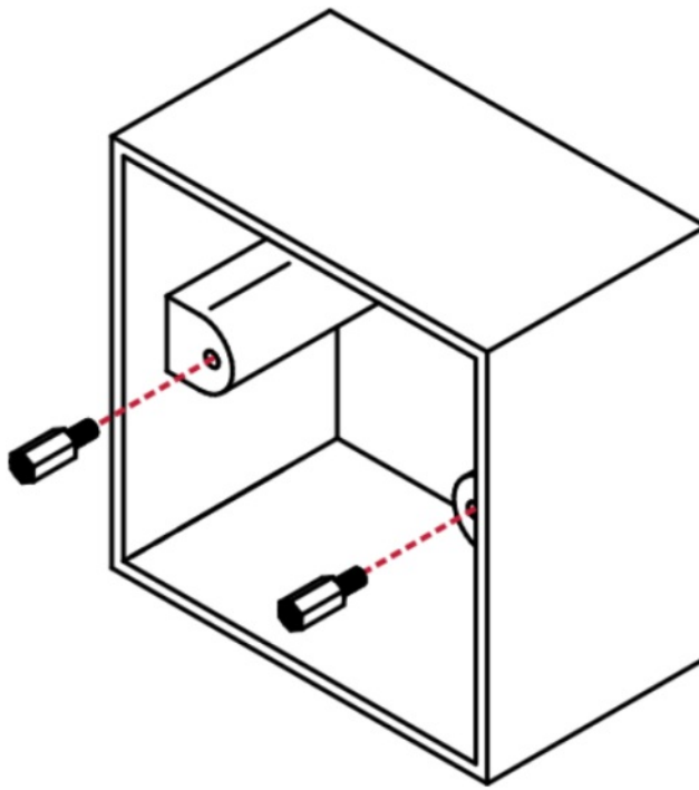
Figure 12: Using Spacers for BS-EN 60670-1 Junction Box
