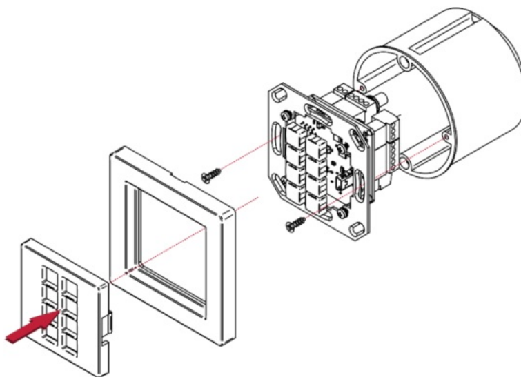
Figure 11: Installing the RC-308 EU/UK Version
