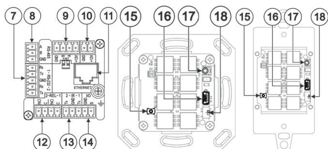
Figure 3: Ethernet and K-NET Control Keypad Rear View
