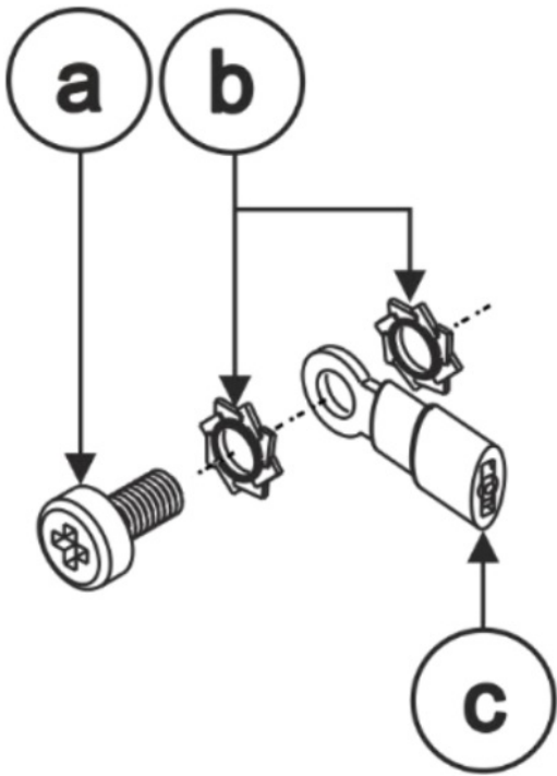
Figure 10: Grounding Connection Components
