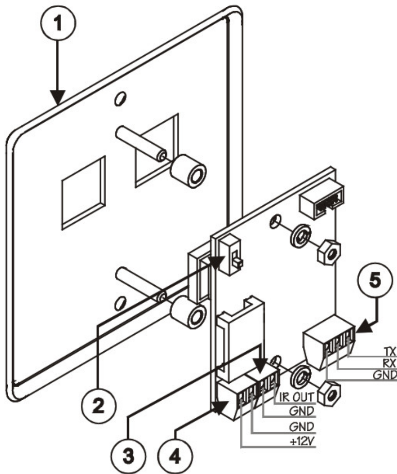
Figure 2: RC-2C Rear Panel
