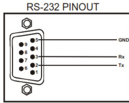
Figure 4: RS-232 PINOUT Connection
