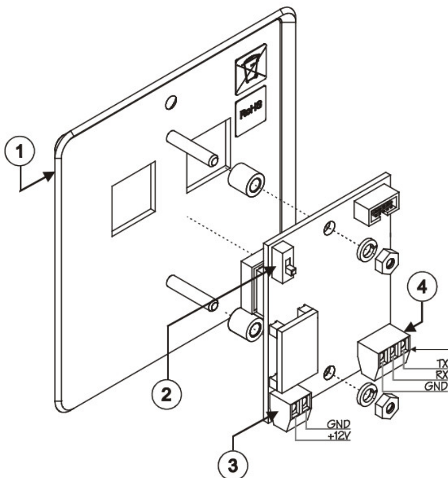
Figure 3: RC-2 Rear Panel
