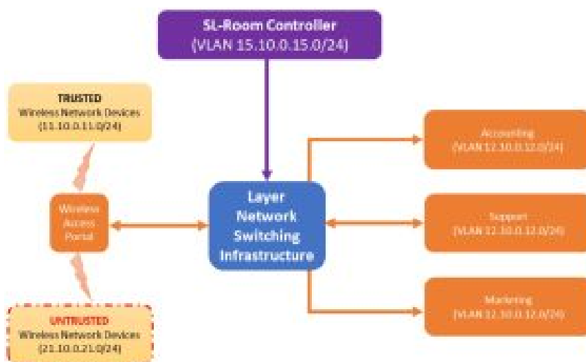
Figure 2: Segmented Network
