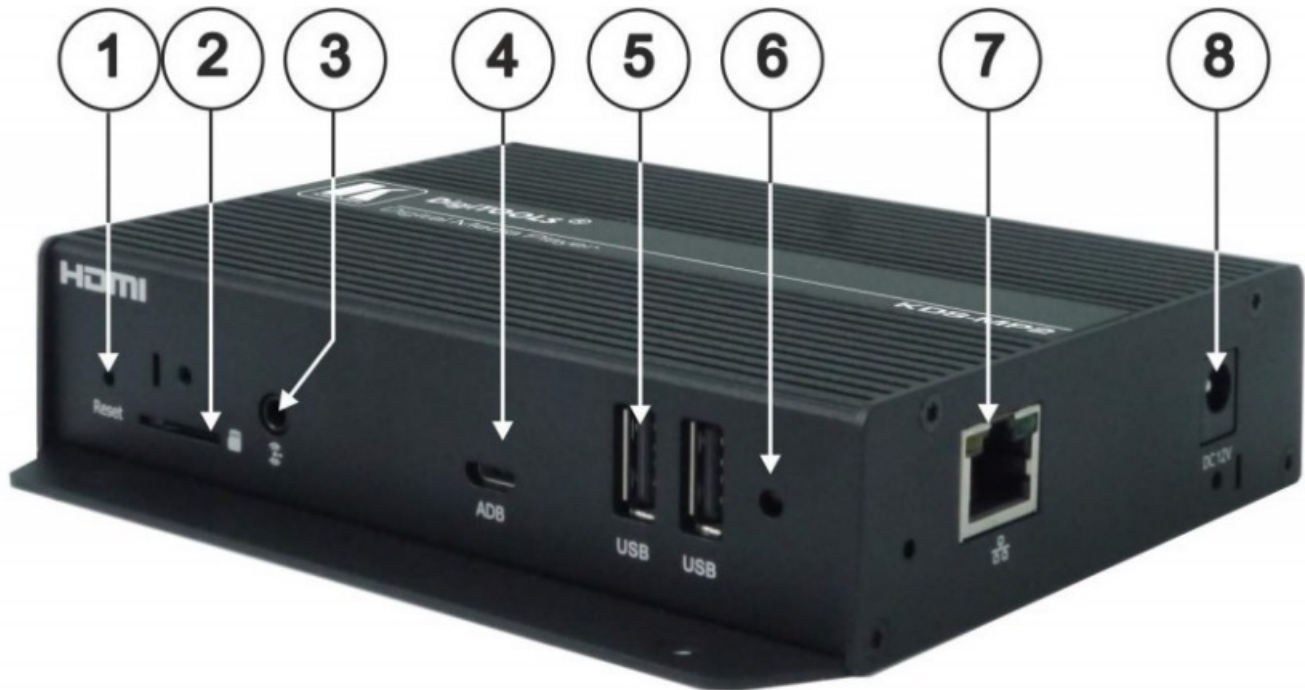
Figure 1: KDS-MP2 Digital Media Player – Front
