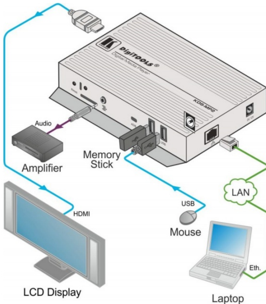
Figure 3: Connecting the KDS-MP2 Digital Media Player
