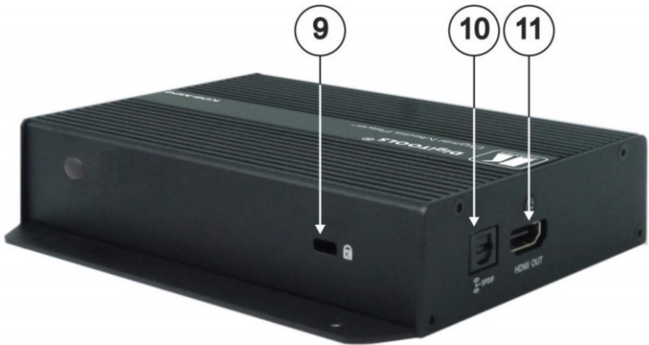
Figure 2: KDS-MP2 Digital Media Player – Rear
