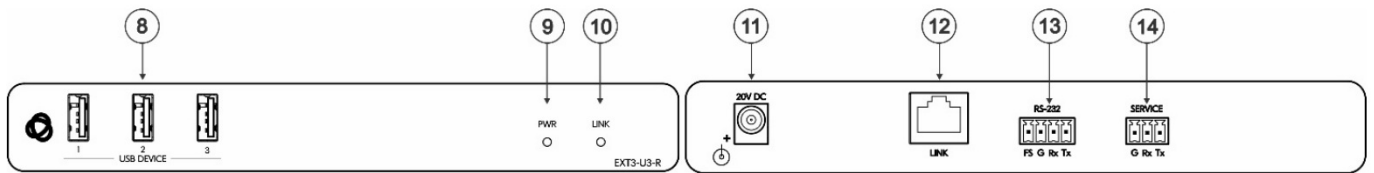
Figure 2: EXT3-U3-R Receiver
