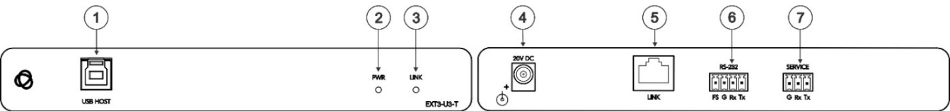
Figure 1: EXT3-U3-T Transmitter
