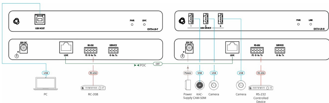
Figure 3: Connecting to the EXT3-U3-T/R
