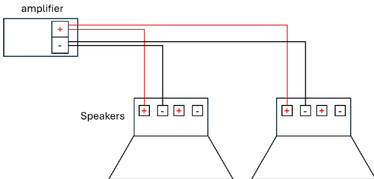
Figure 4 -Parallel Wiring - Separate Cables
