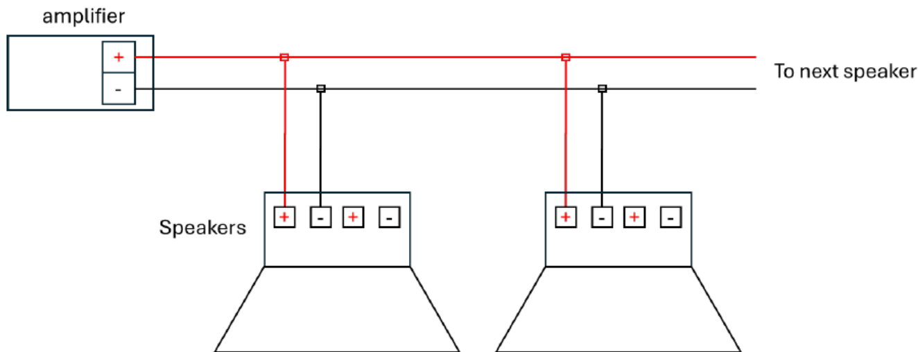
Figure 3 - Parallel Wiring
