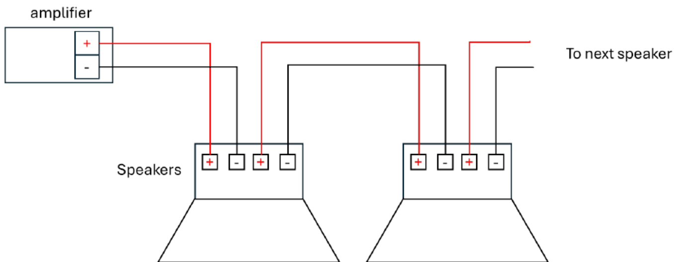
Figure 5 - Daisy Chain Wiring
