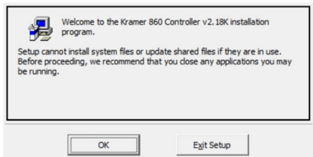
Figure 1: Installation Prompts
