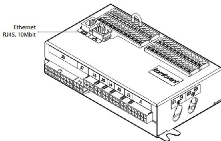
Picture 1. C5 controller board
