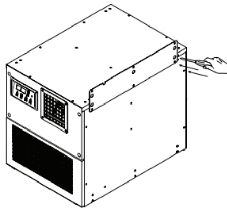
Figure 20 - braket attachment
