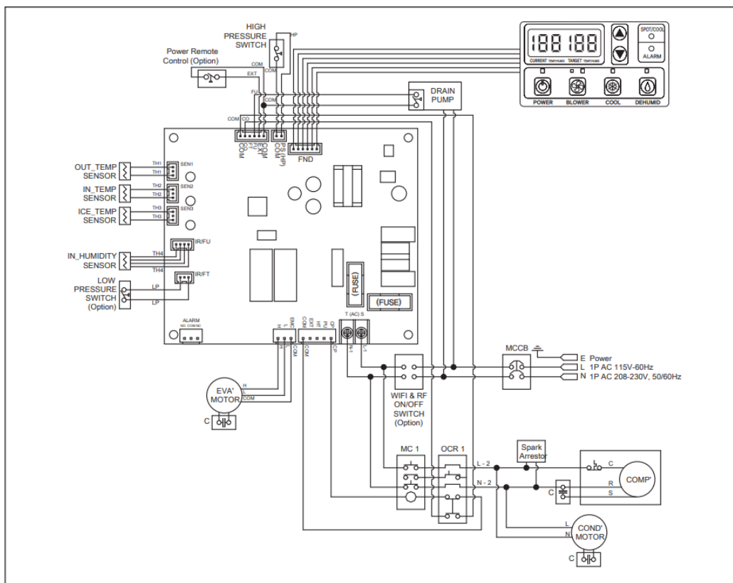
Figure 26 - Circuit Wiring Diagram
