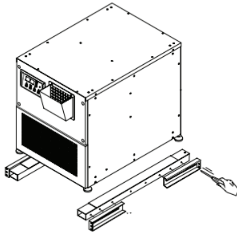
Figure 11- rack assembly attachment
