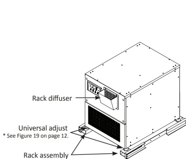
Figure 9 - server rack kit attachment
