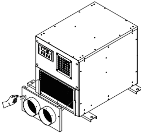
Figure 16 - eva flange attachment
