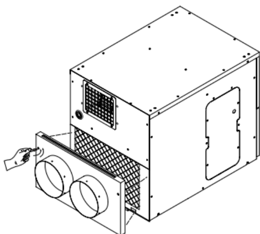
Figure 24 - Removing condenser Filters
