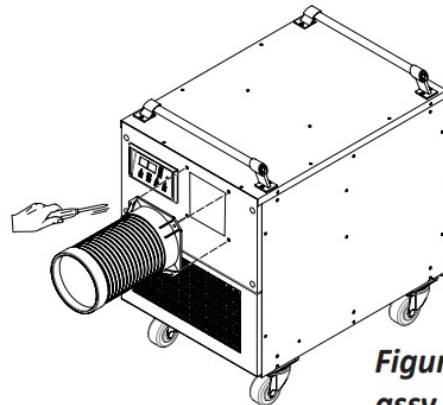
Figure 5 - portable kit attachment
