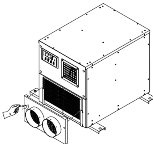
Figure 25 - Removing evaporator Filters
