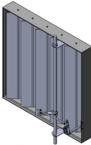
jackshaft mounting
