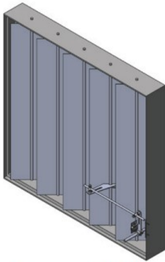
damper blade mounting
