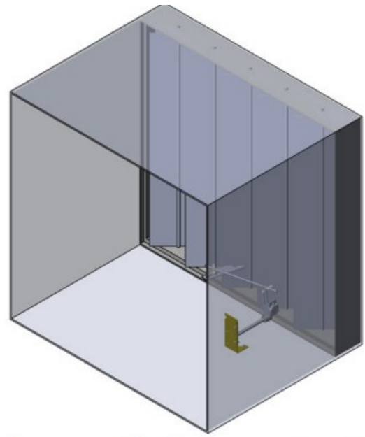
damper blade mounting in a duct with VTD-0903
