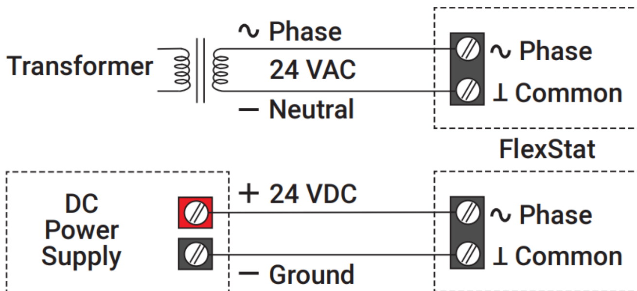
Illustration 12—Power Terminals
