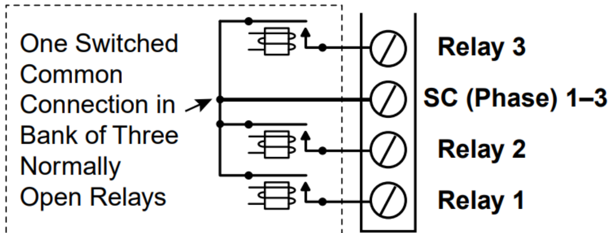
Illustration 11—Switched (Relay) Common and Relay Bank
