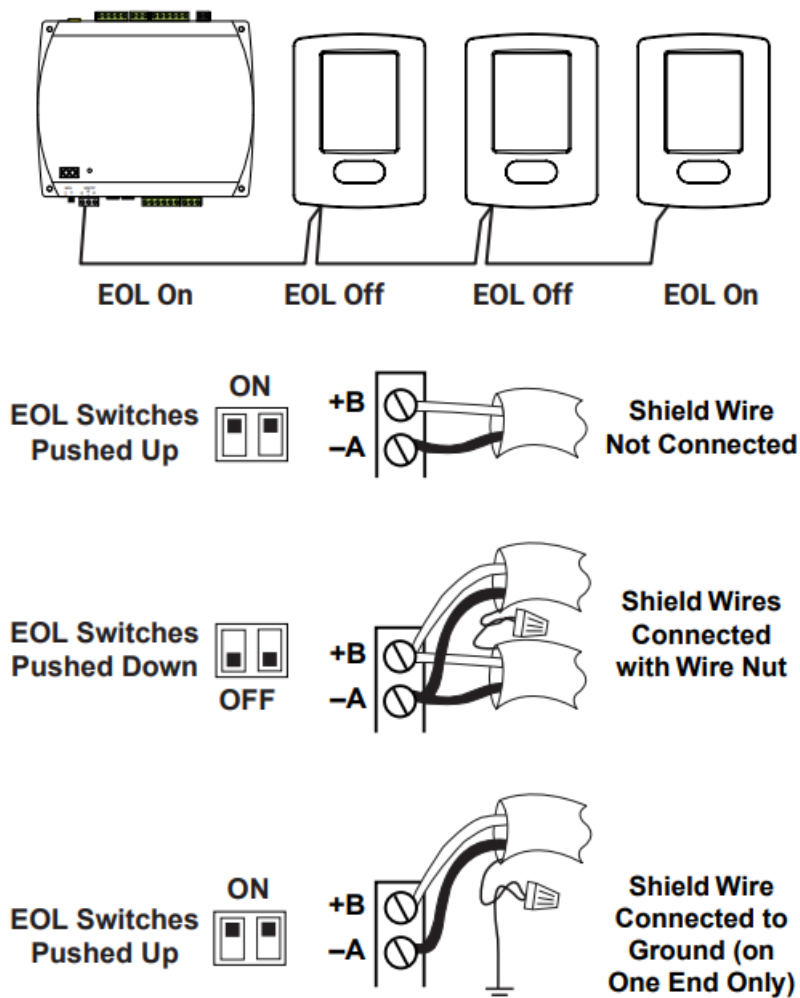
Illustration 10—MS/TP Connections and EOL (MS/TP Models)
