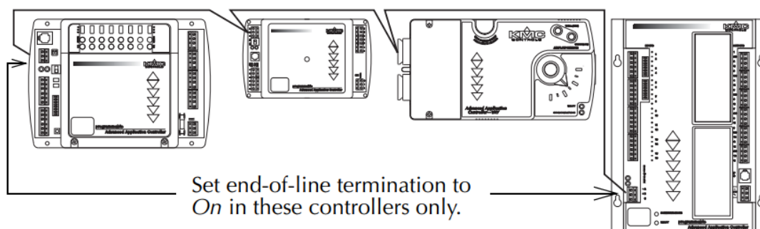
Illustration 2-5 End of line termination
