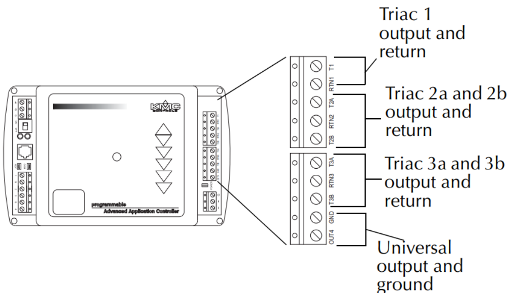
Illustration 2-2 Output terminals
