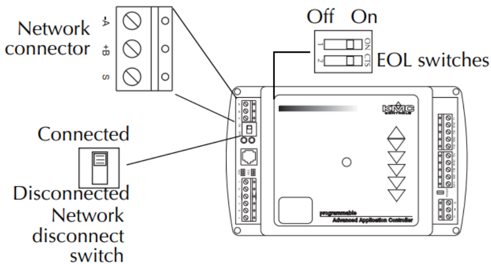
Illustration 2-6 Location of EOL switch
