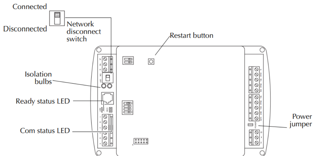
Illustration 3-1 Controls and indicators
