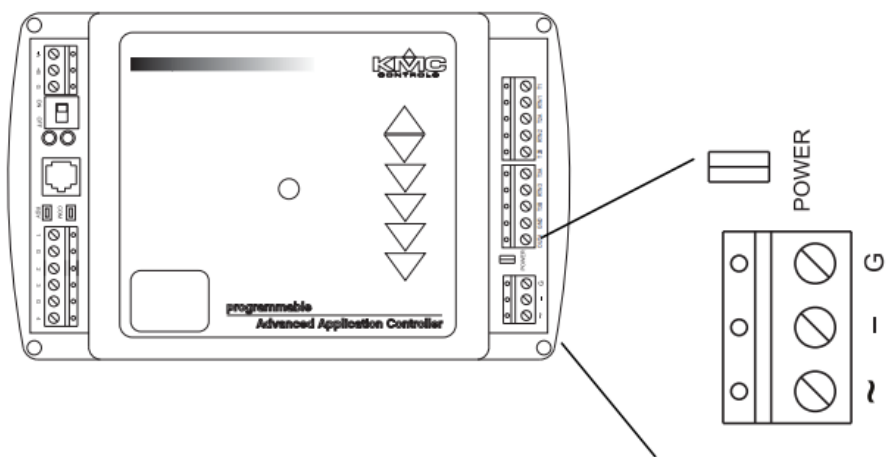
Illustration 2-7 Power terminal and jumper
