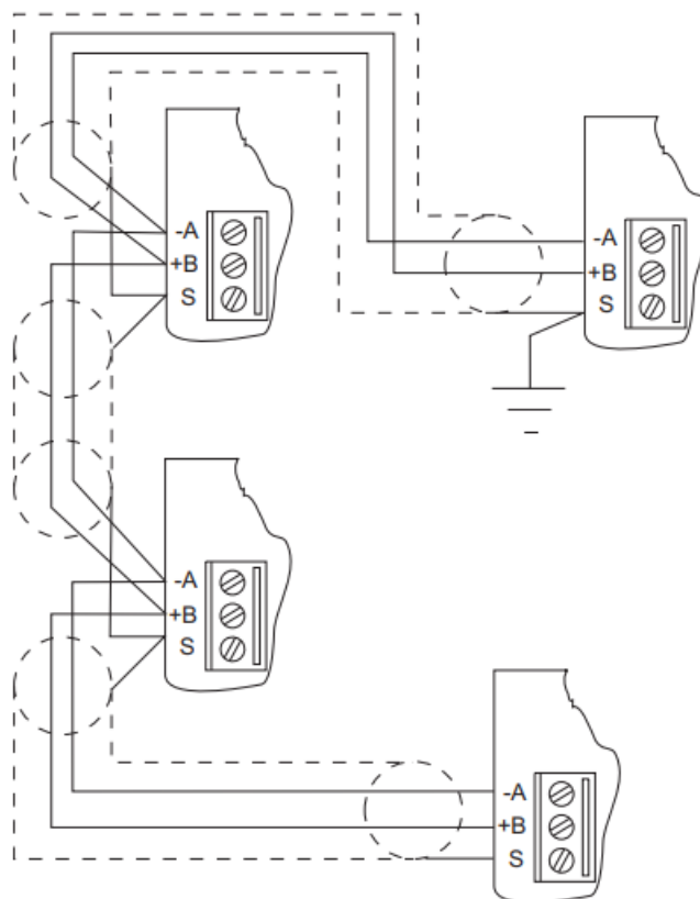
Illustration 2-4 MS/TP network wiring
