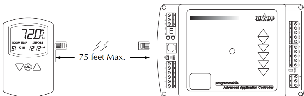
Illustration 2-3 Connection to a NetSensor
