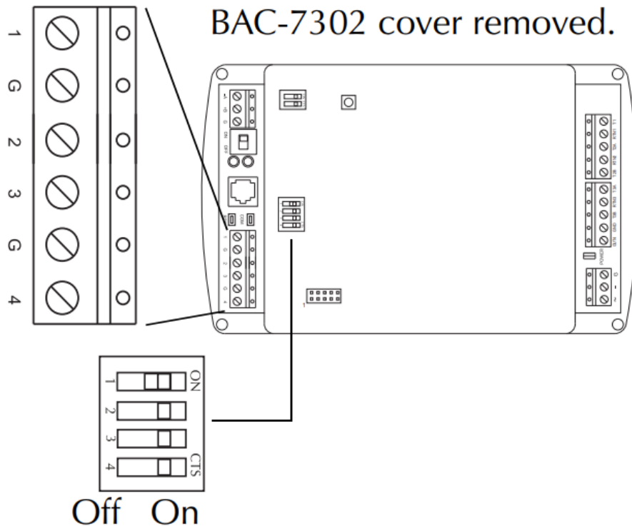
Illustration 2-1 Pull-up resistors and input terminals
