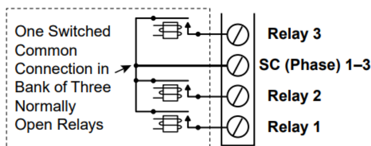
Illustration 11—Switched (Relay) Common and Relay Bank
