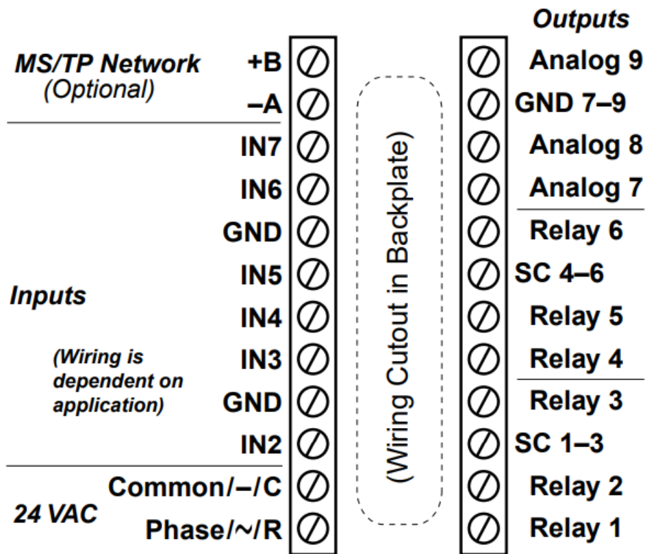
Illustration 5—BAC-19xx63 Terminals and Connections
