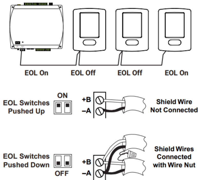
Illustration 10—MS/TP Connections and EOL (MS/TP Models)
