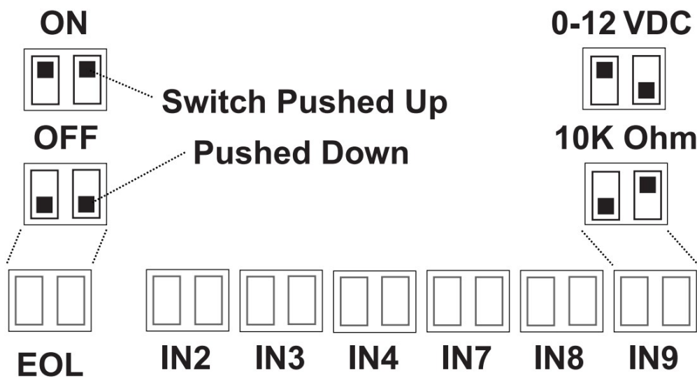
Illustration 4—BAC-13xxxx/14xxxx Switch Positions
