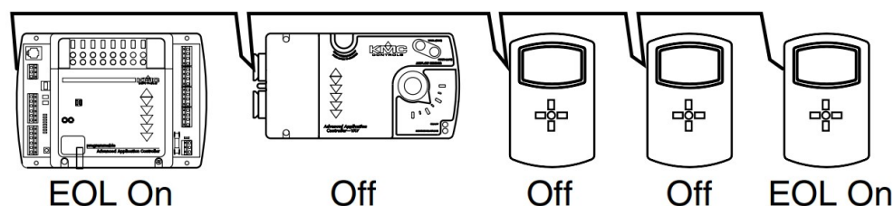
Illustration 2—MS/TP Network End-Of-Line Termination
