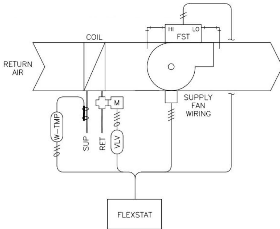
FCU—4 Pipe, Modulating
