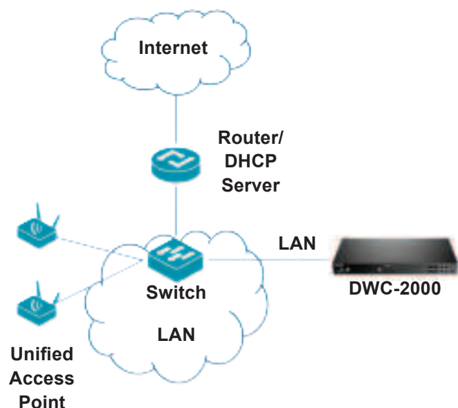
Figure 10. Network Topology
