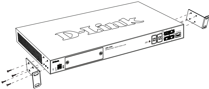
Figure 5. Mounting Brackets
