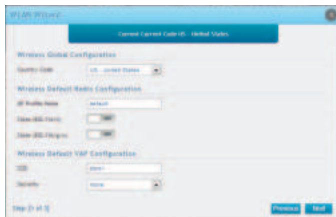
Figure 13. WLAN Wizard
