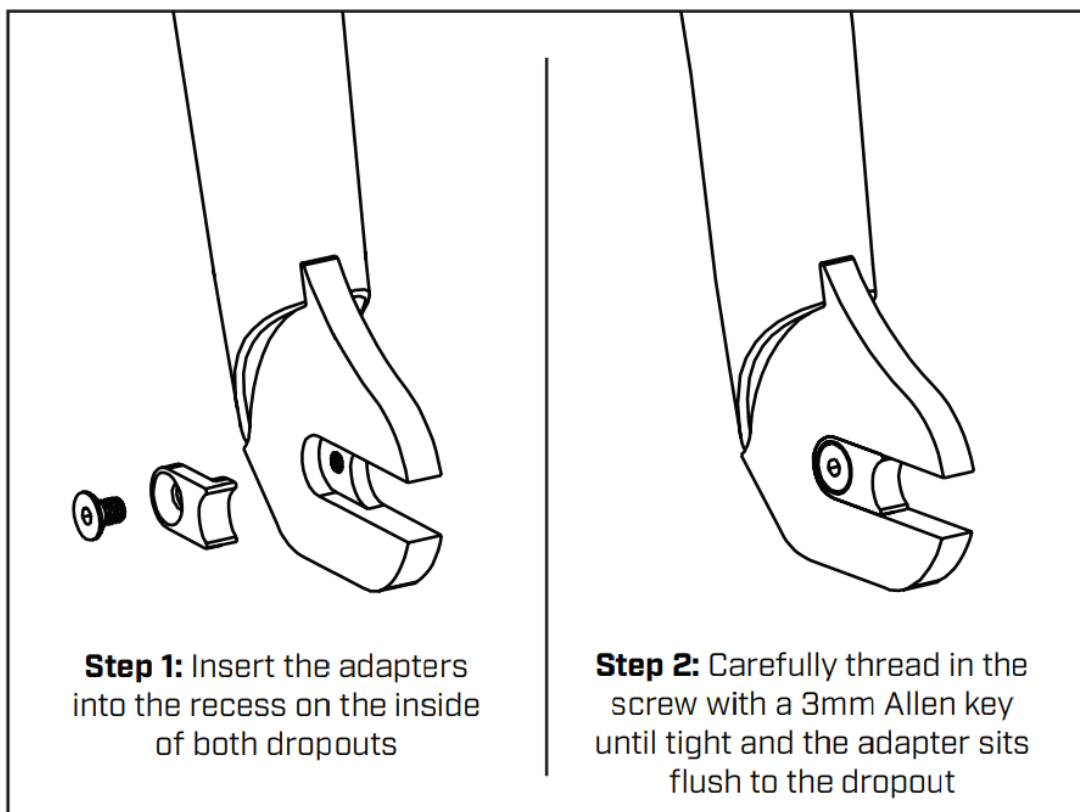
FIG. 2 - OFFSET ASSEMBLY
