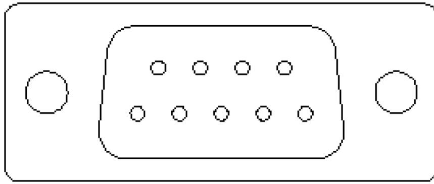
Figure 10: standard RS232 interface
