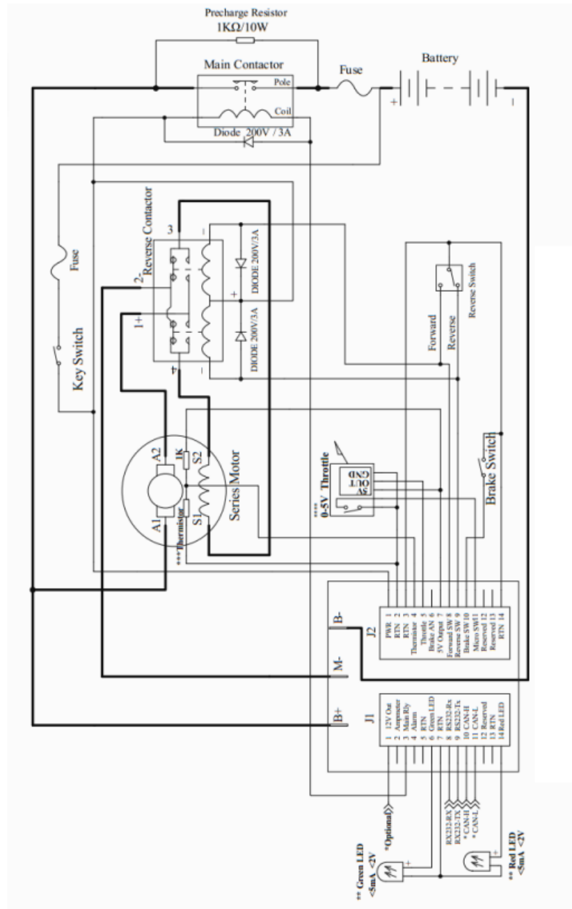
Figure 6: KDZ/KDZ-E series motor controller standard wiring
