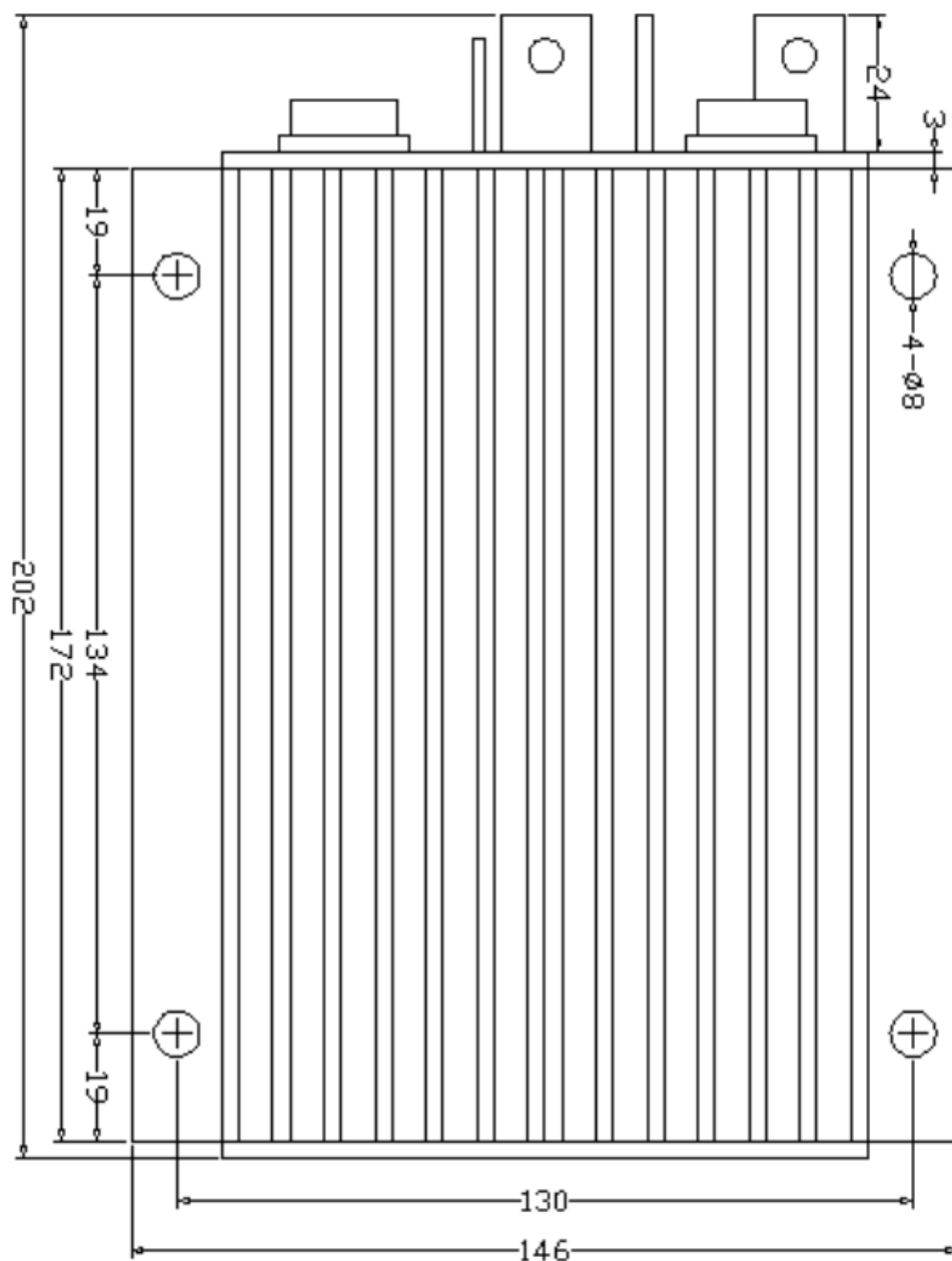
Figure 1: KDZ mounting holes' dimensions (dimensions in millimeters)
