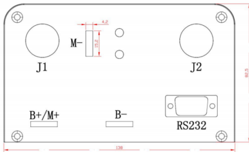
Figure 4: Front panel of KDZ-E motor controller
