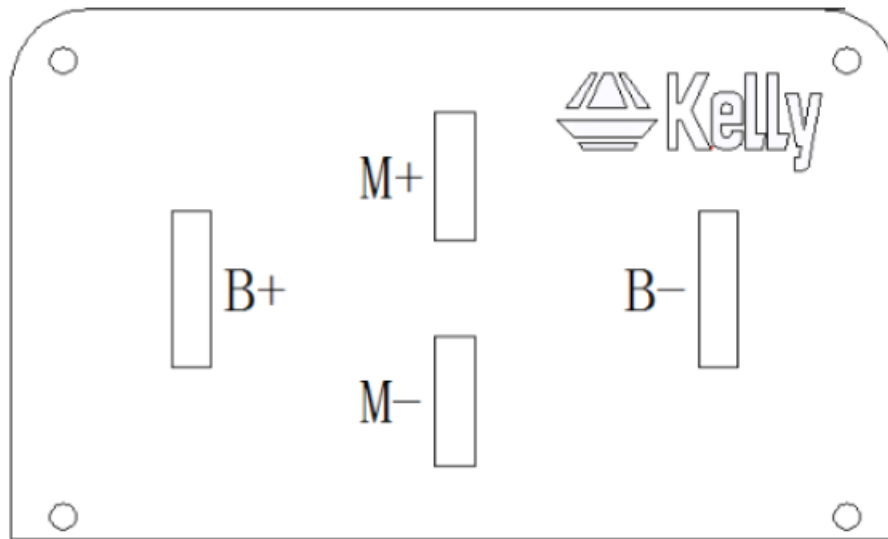
Figure 3: Front panel of HPM motor controller
