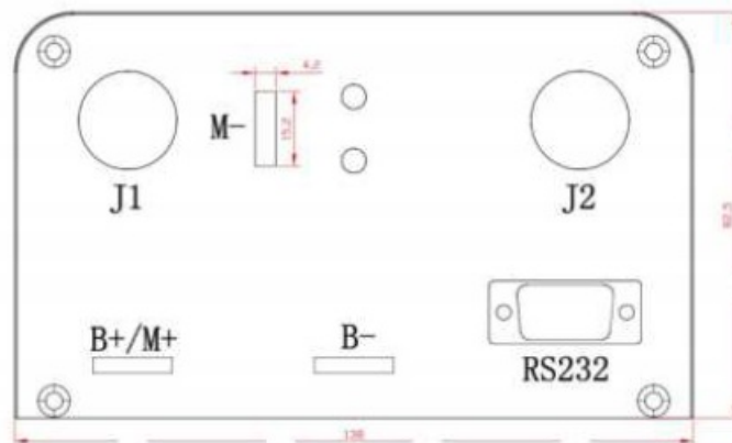
Figure 3: Front panel of KDZ motor controller
