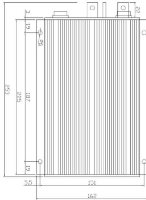
Figure 2: KDZ-E mounting holes' dimensions (dimensions in millimeters)
