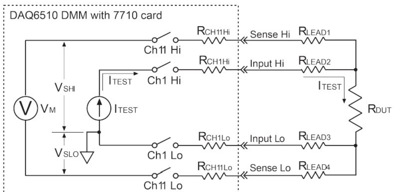
Figure 11: Low-ohms measurements using 4-wire method
