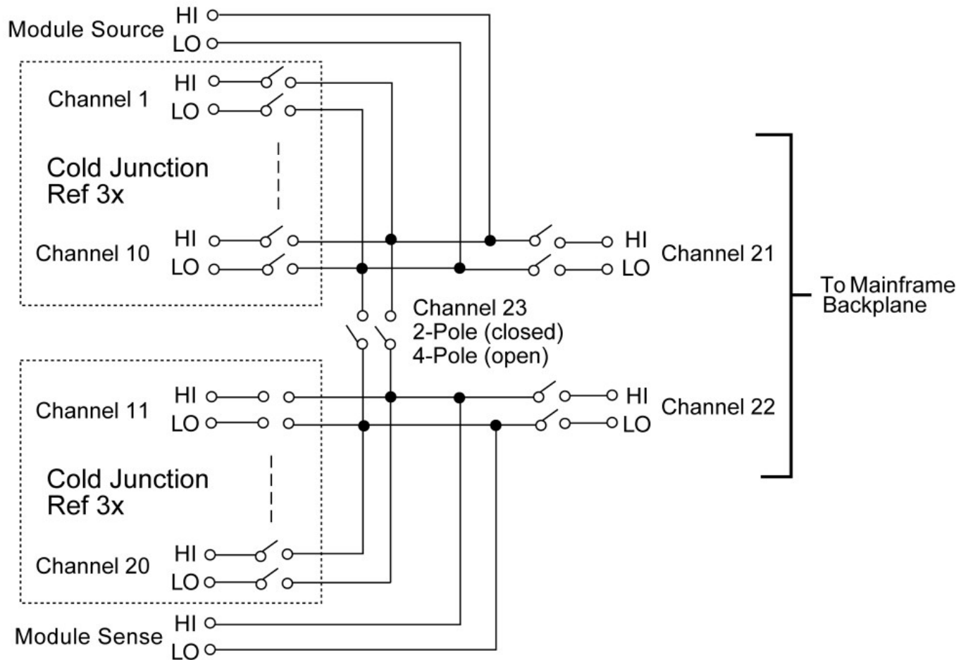
Figure 6: 7710 simplified schematic
