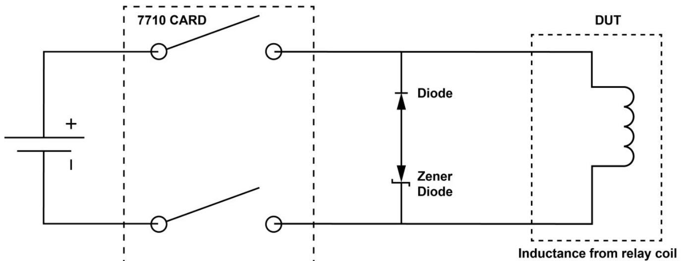
Figure 14: Diodes at relay coil to clamp spikes
