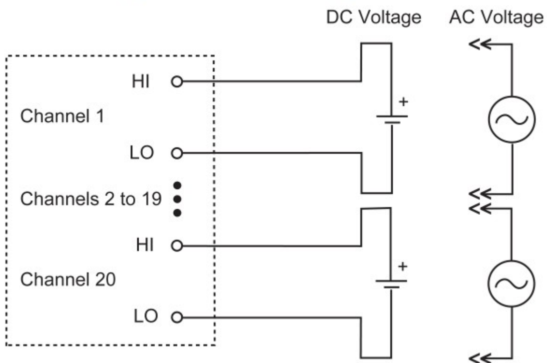
Figure 10: DC or AC voltage connections
