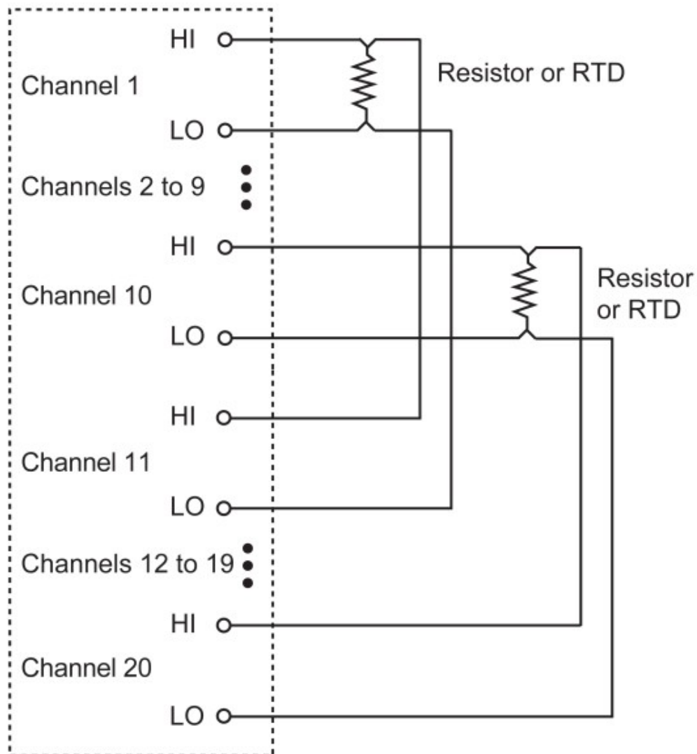
Figure 9: Four-wire resistance and RTD connections
