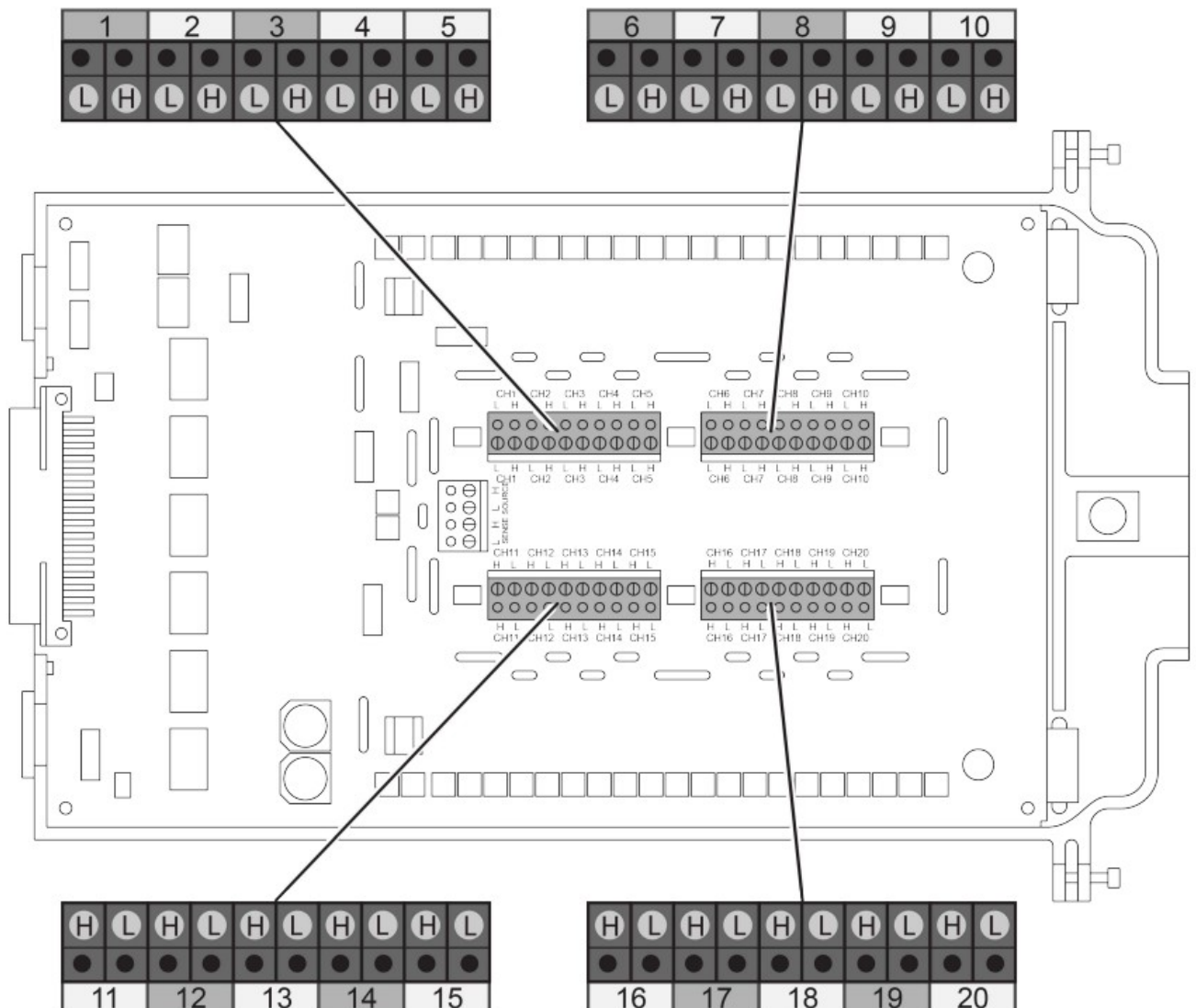
Figure 4: Screw terminal channel designations
