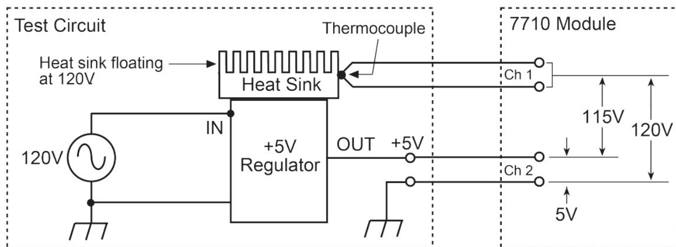
Figure 12: Example of an unsafe measurement practice
