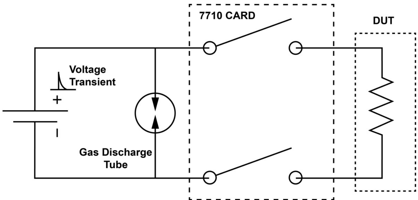
Figure 15: Gas discharge tube clamp
