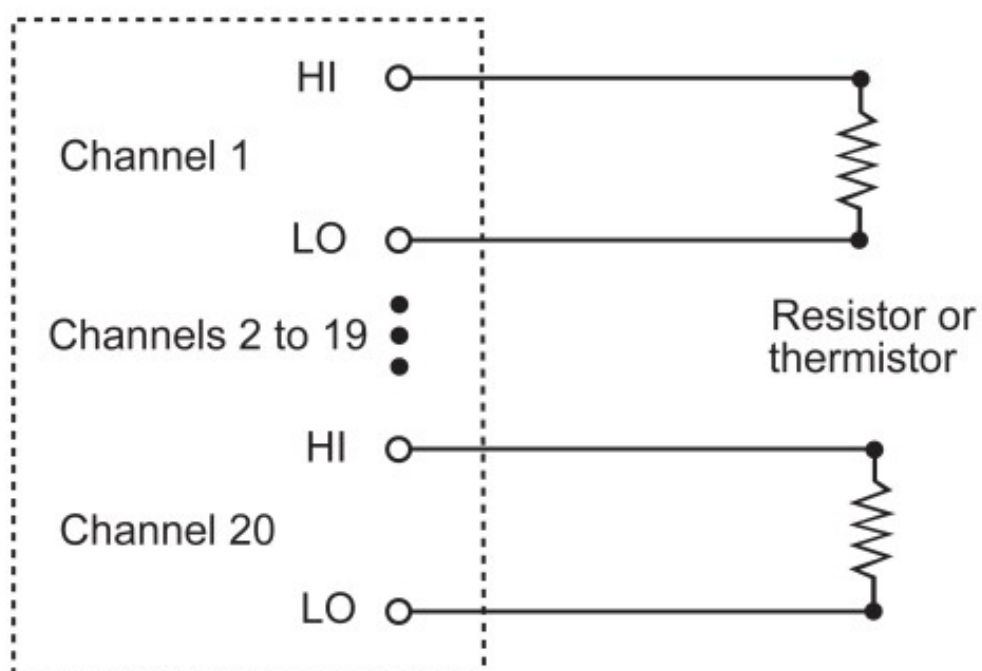
Figure 8: Two-wire resistance and thermistor connections
