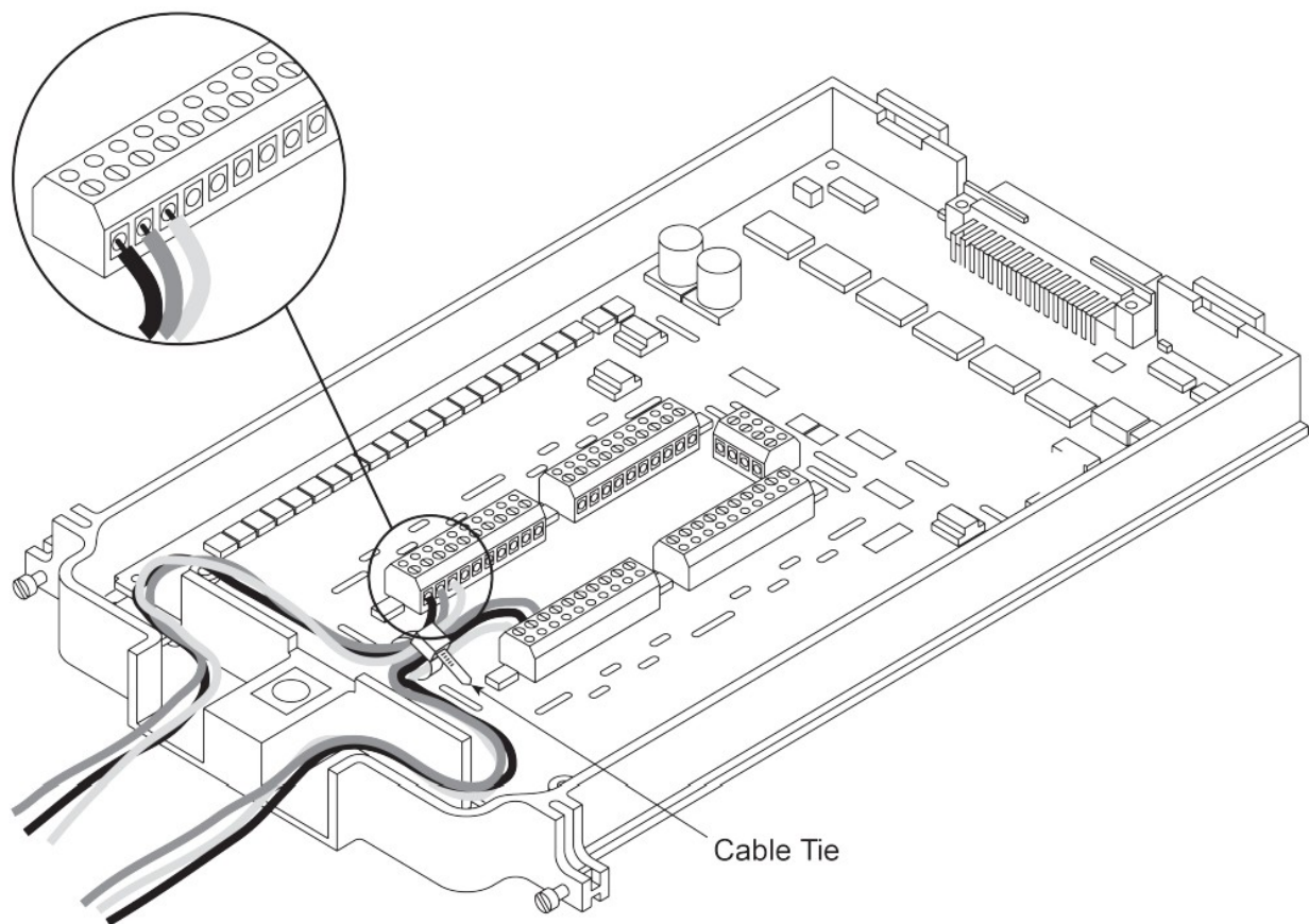
Figure 5: Wire dressing
