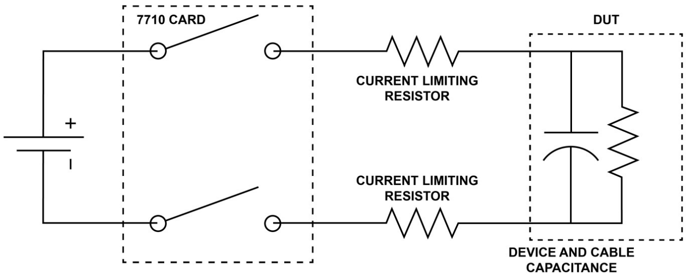
Figure 13: Solid state relay limiting resistor
