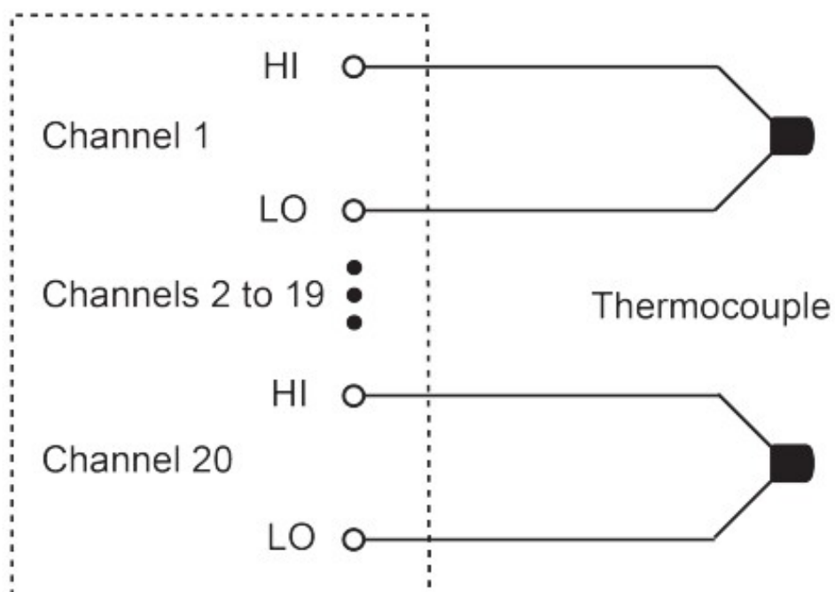
Figure 7: Thermocouple connections
