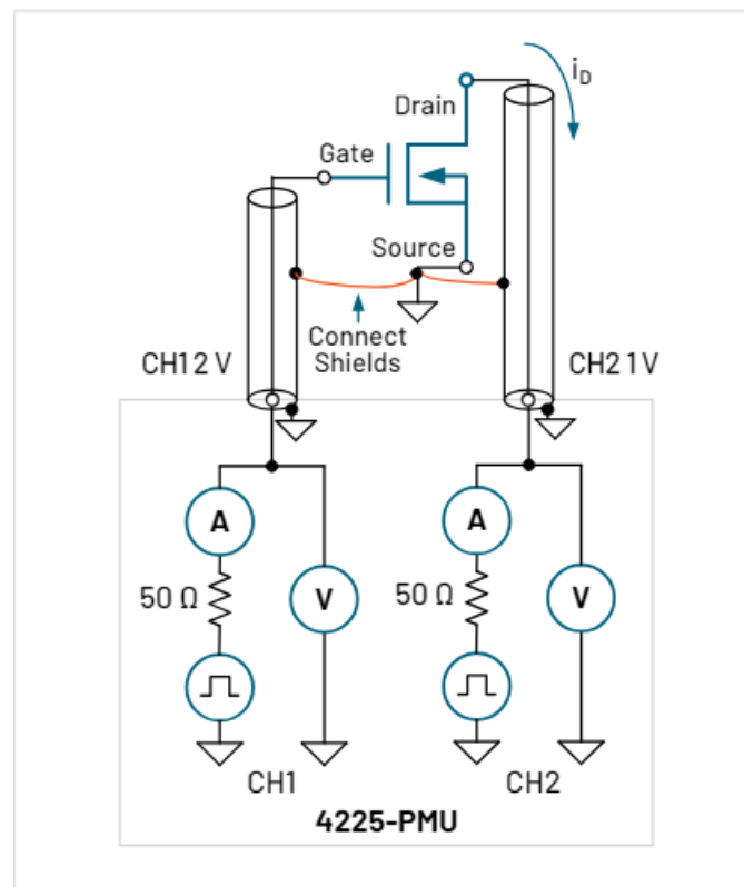
Figure 7. Connections from the two channels of the PMU to a three-terminal MOSFET.
