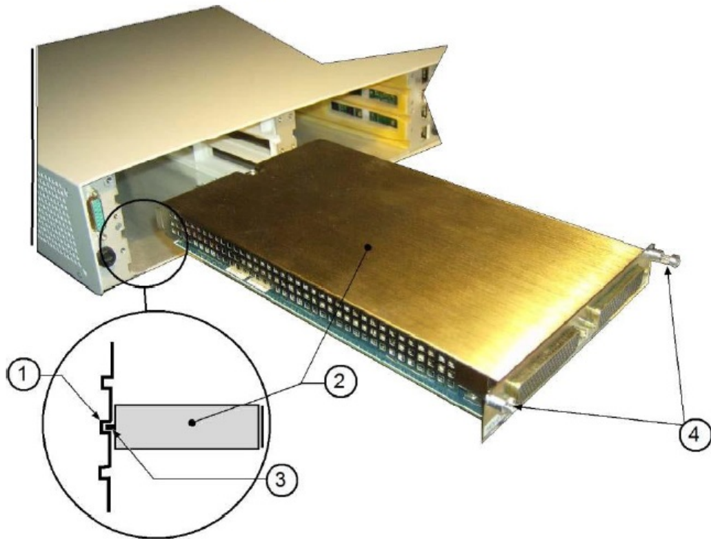
Figure 2: Module installation
