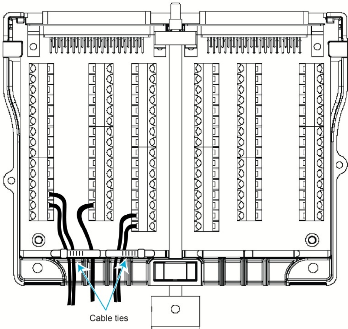
Figure 10: Routing and securing cables with ties
