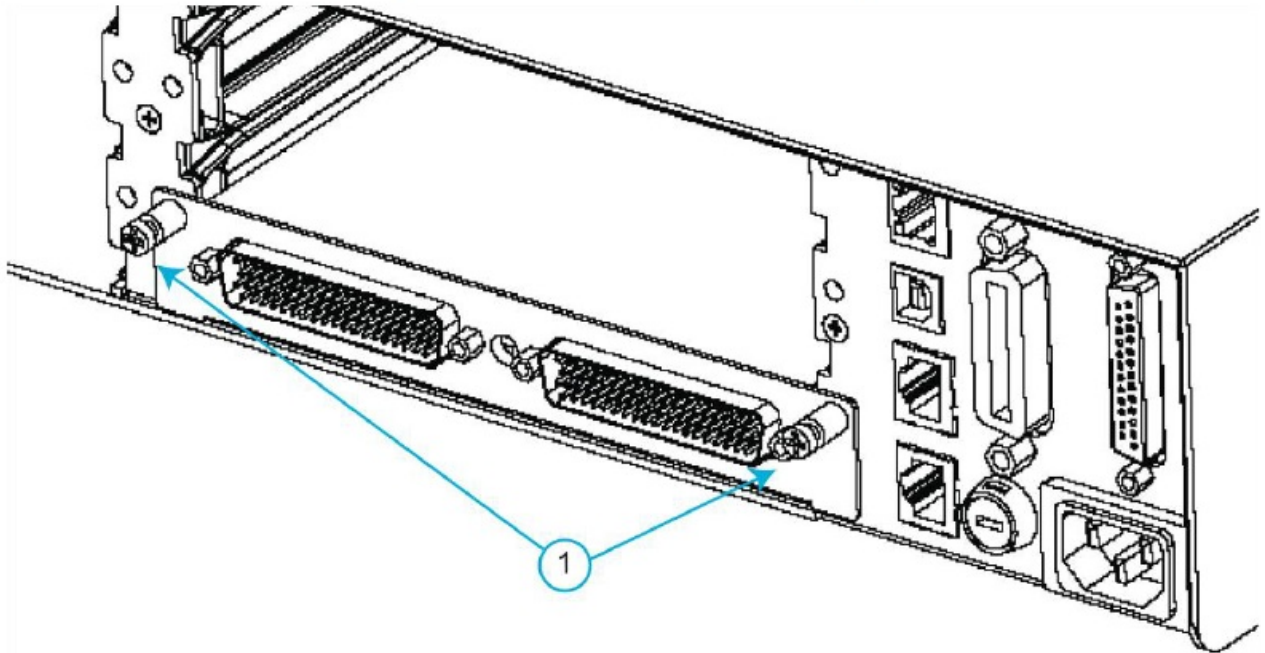
Figure 12: Check 3700A card mounting screws
