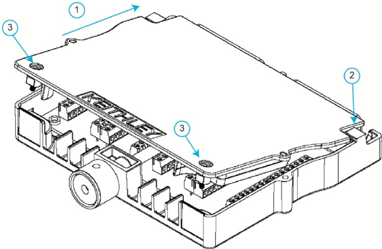
Figure 11: Install the screw-terminal assembly top cover
