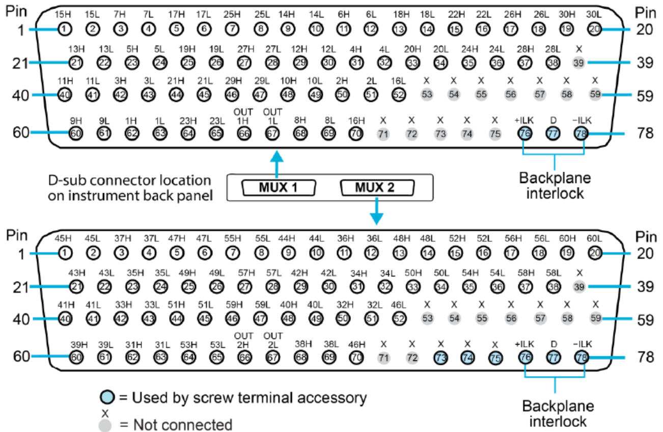
Figure 3: Model 3723 D-sub connections in 2-pole mode
