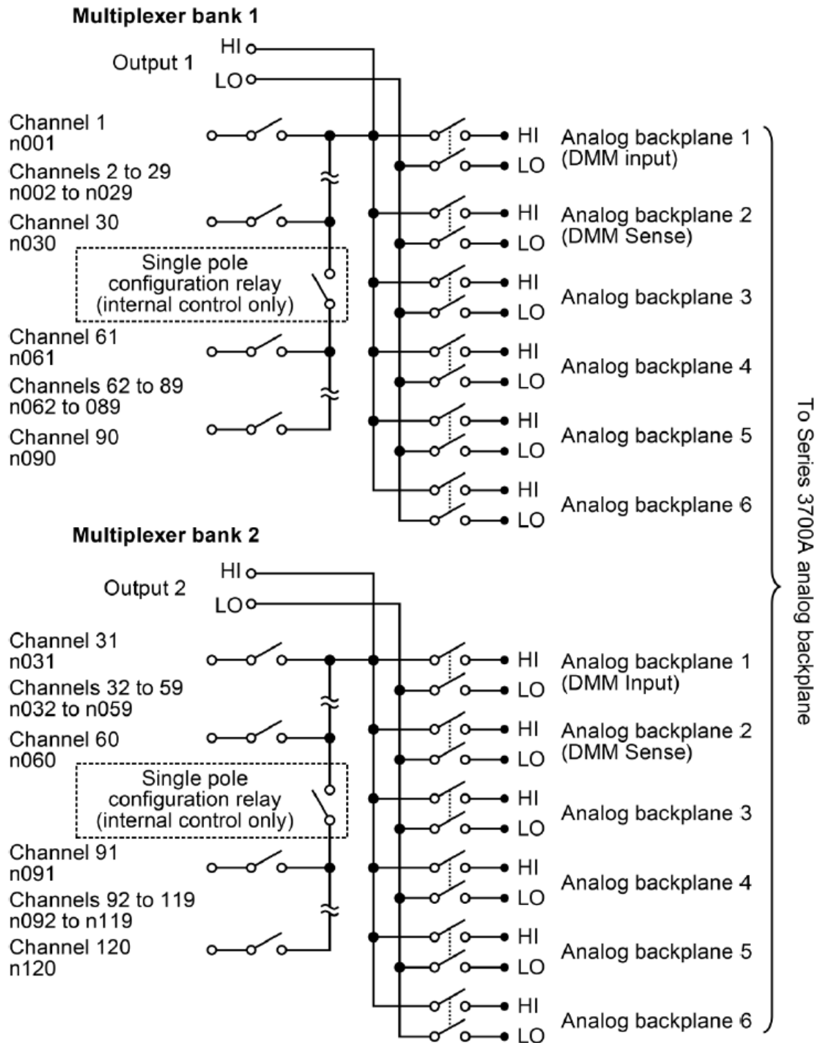
Figure 6: Model 3723 schematic single-pole mode
