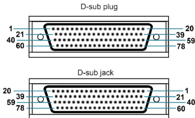
Figure 15: Model 3720-MTC-3 connectors
