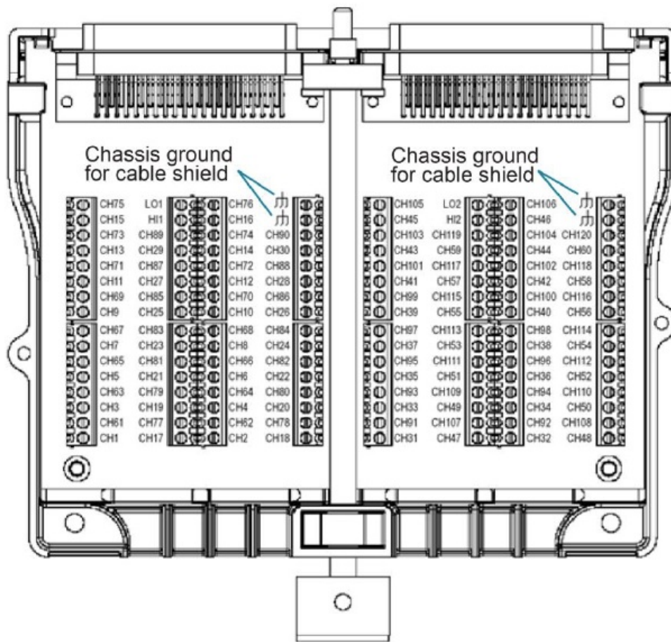
Figure 8: Model 3723-ST-1 Screw-Terminal Accessory
