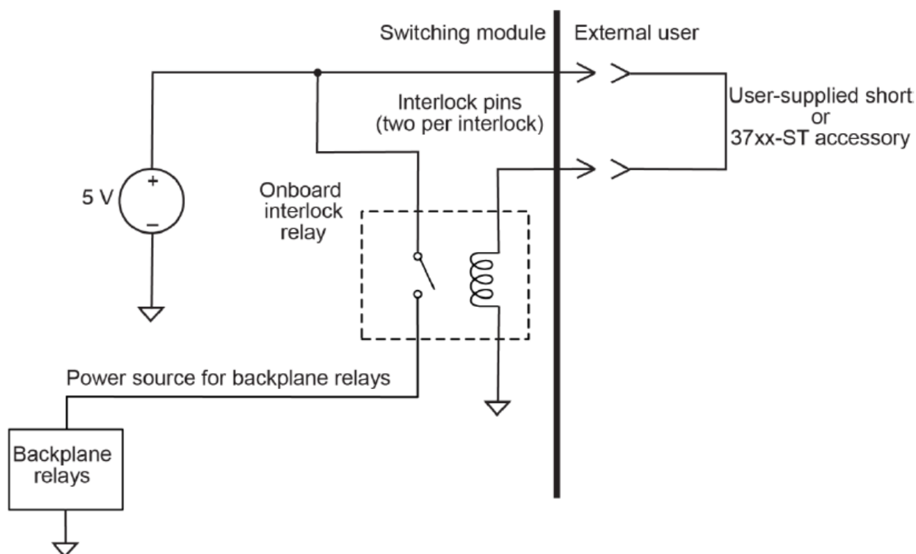
Figure 16: Simplified interlock circuit
