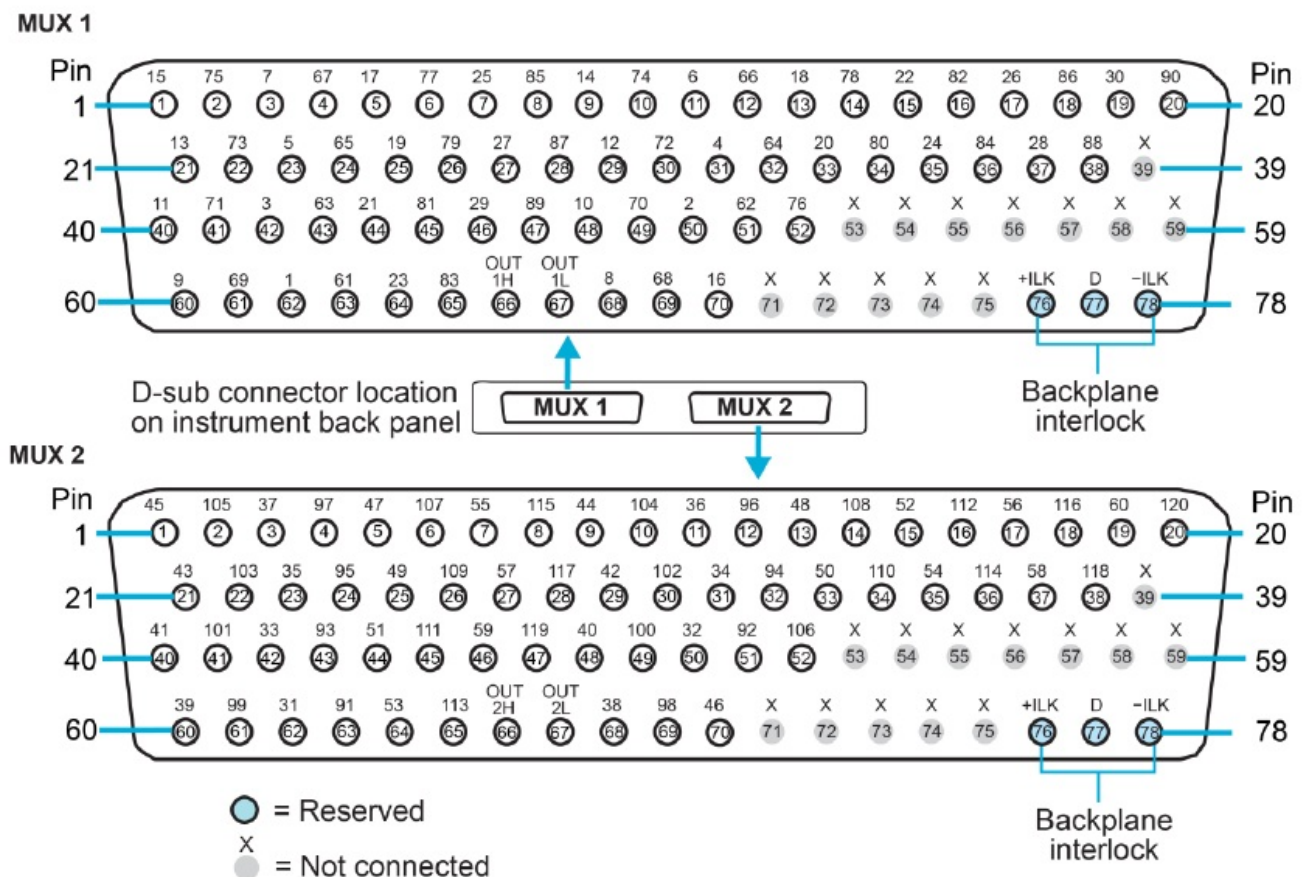
Figure 4: Model 3723 D sub-connections 1-pole
