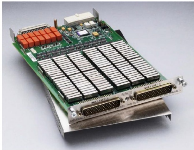
Figure 1: Model 3723 High-Speed 1 x 30 Card
