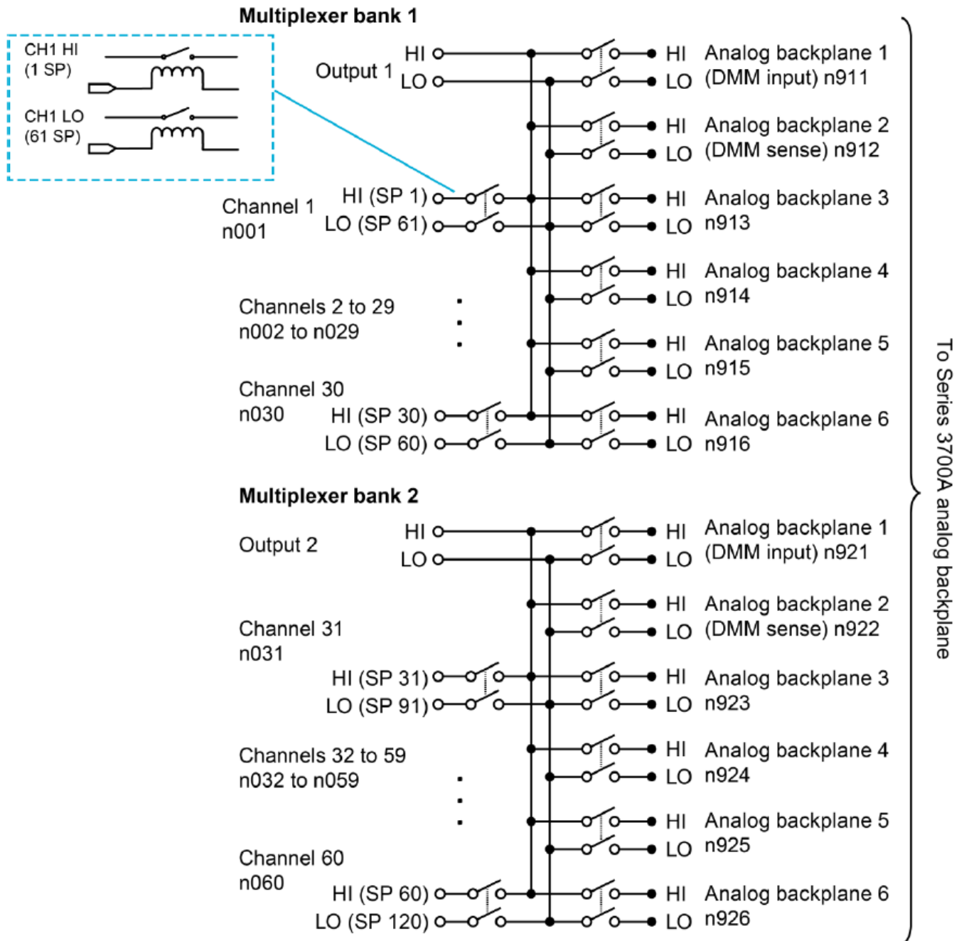
Figure 5: Model 3723 schematic two-pole mode
