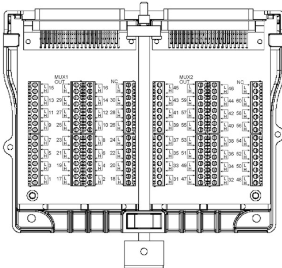
Figure 7: Model 3723-ST Screw-Terminal Accessory
