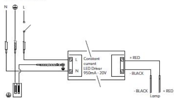
ON-OFF wiring diagram
