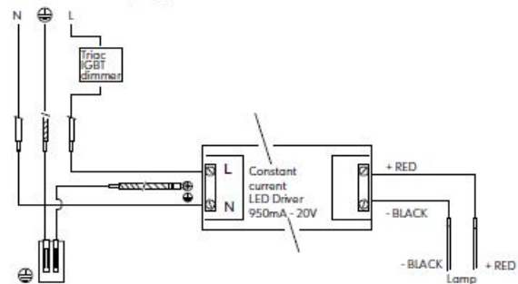
PHASE CUT DIMM wiring diagram
