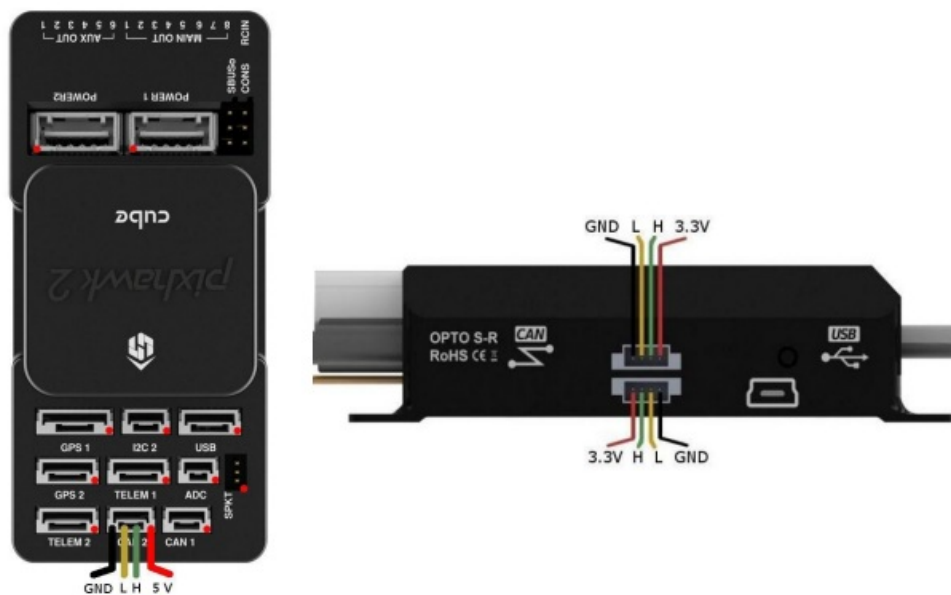
Figure 1: Pixhawk 2.1 (CUBE) & ESC wiring pins.
