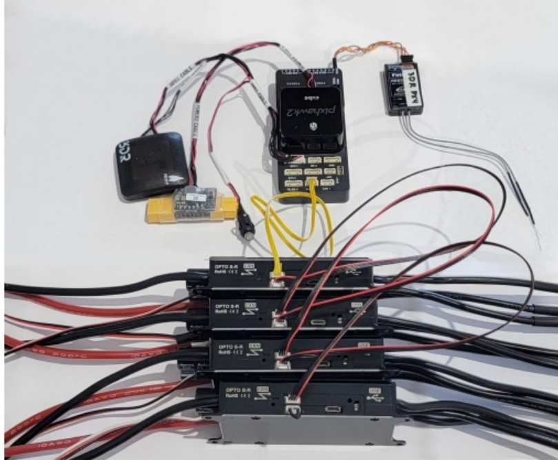
Figure 1: CAN bus wiring.
