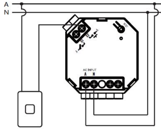
FUNCTION 2 - MOMENTARY SWITCH INPUT
