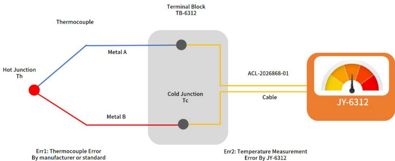
Figure 3 Thermocouple Temperature Measurement Principle
