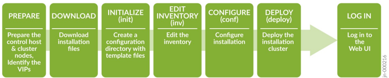
Figure 1: High-Level Process Flow for Installing Paragon Automation
