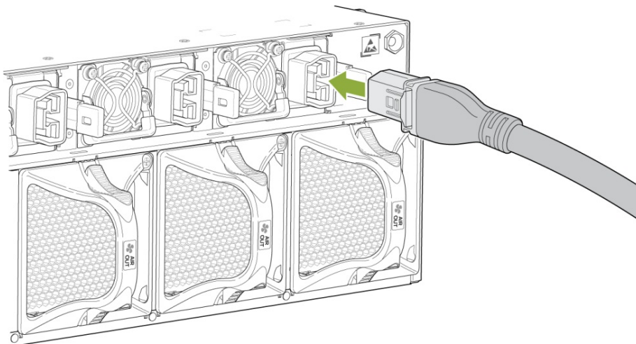
Figure 11: Connecting an AC/HVDC Power Cord (PTX10003-80C)
