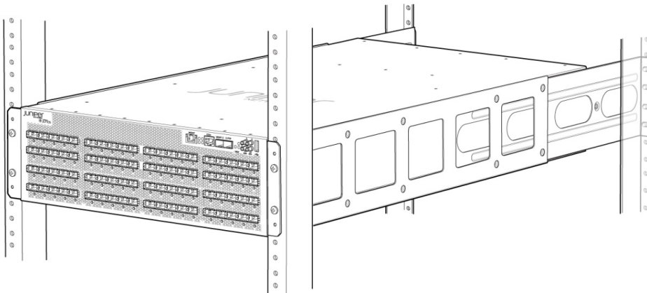
Figure 5: Securing the Side Rails ( PTX10003-80C)
