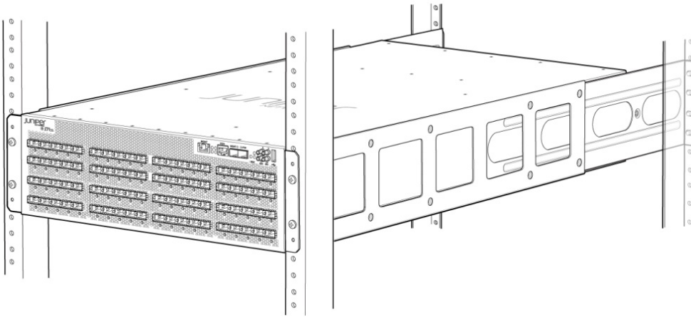
Figure 7: PTX10003 Secured in Rack (PTX10003-80C)
