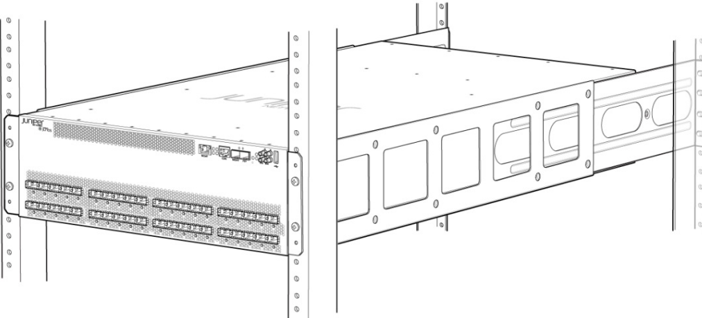
Figure 7: PTX10003 Secured in Rack (PTX10003-80C)
