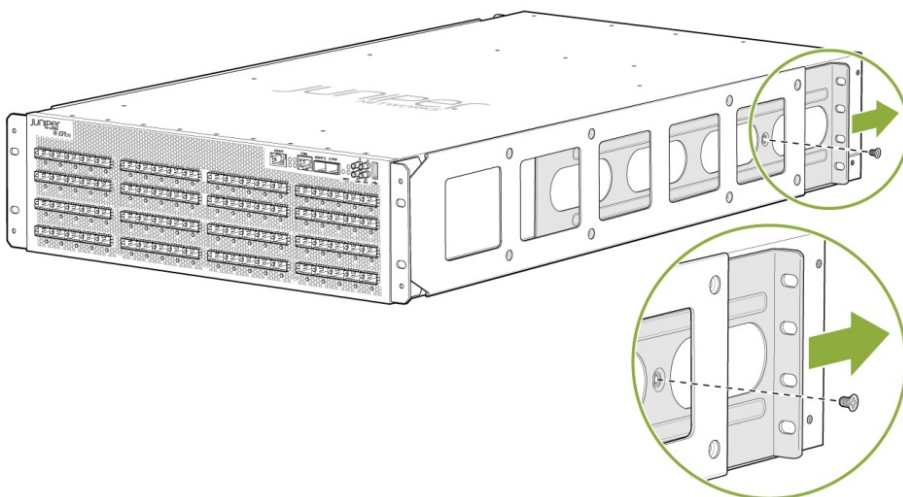
Figure 3: Removing the Slide Rail Screw (PTX10003-80C)
