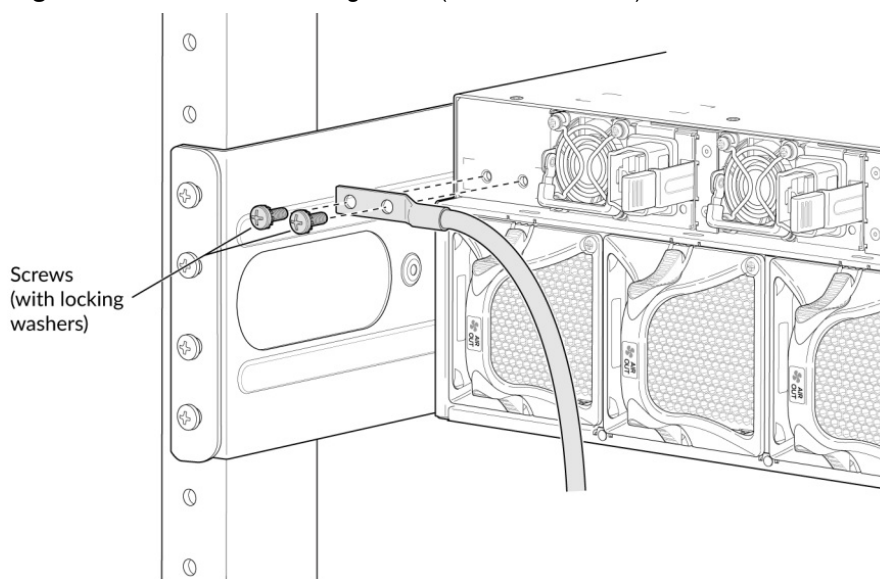
Figure 9: Chassis Grounding Point (PTX10003-80C)
