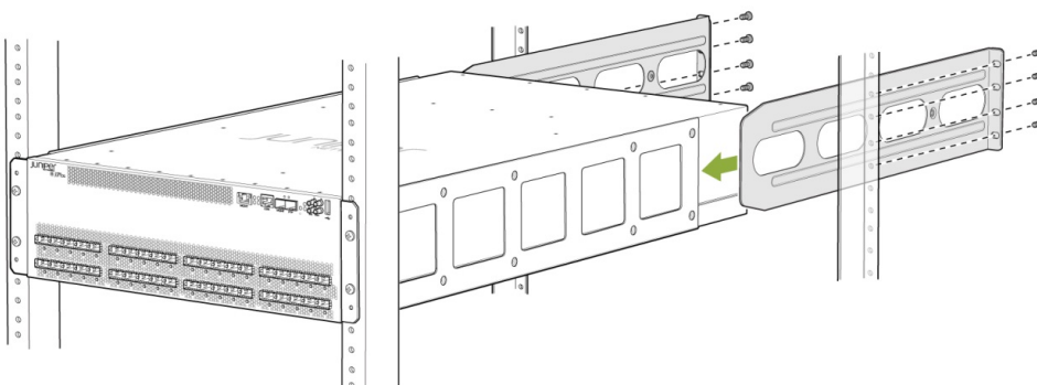
Figure 5: Securing the Side Rails ( PTX10003-80C)
