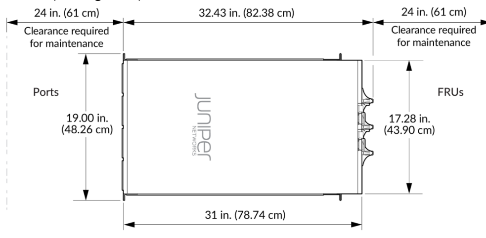
Figure 1: Clearance Requirements for Safety and Hardware Maintenance for the PTX10003
