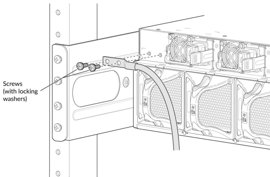
Figure 9: Chassis Grounding Point (PTX10003-80C)
