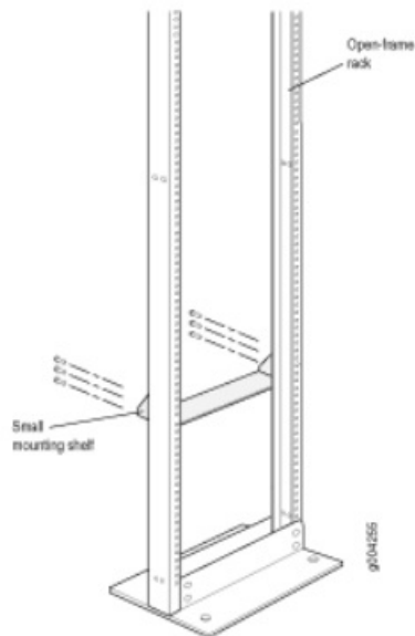
Figure 3: Mounting Hardware for an Open-Frame Rack
