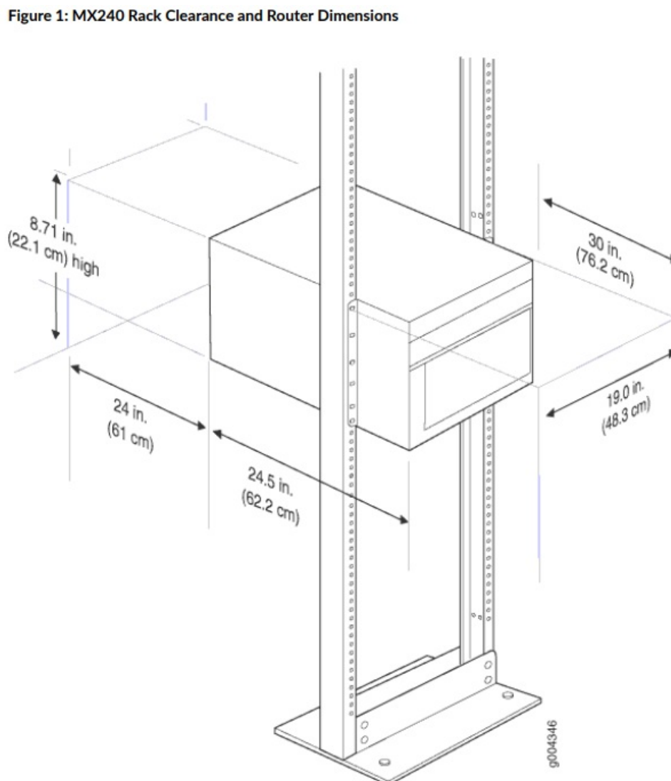
Figure 1: MX240 Rack Clearance and Router Dimensions
