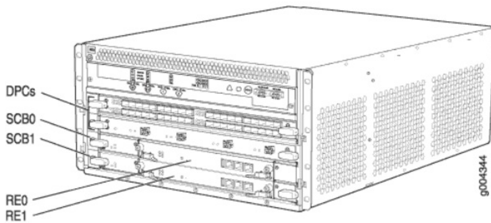
Figure 4: Components to Remove from the Front of the MX240 Router
