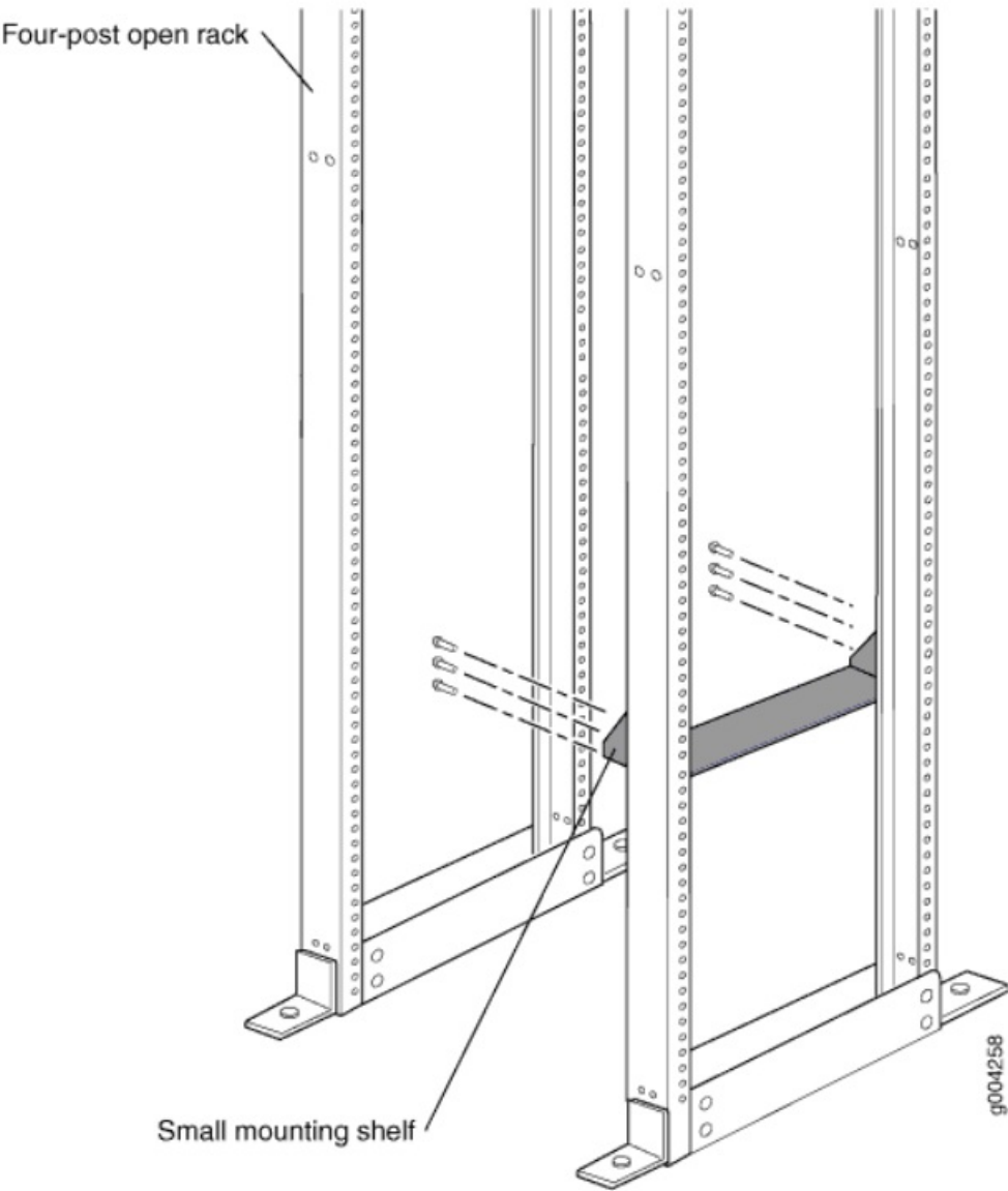
Figure 3: Mounting Hardware for an Open-Frame Rack
