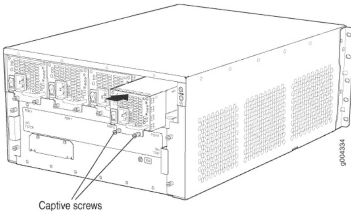
Figure 10: Installing an AC Power Supply
