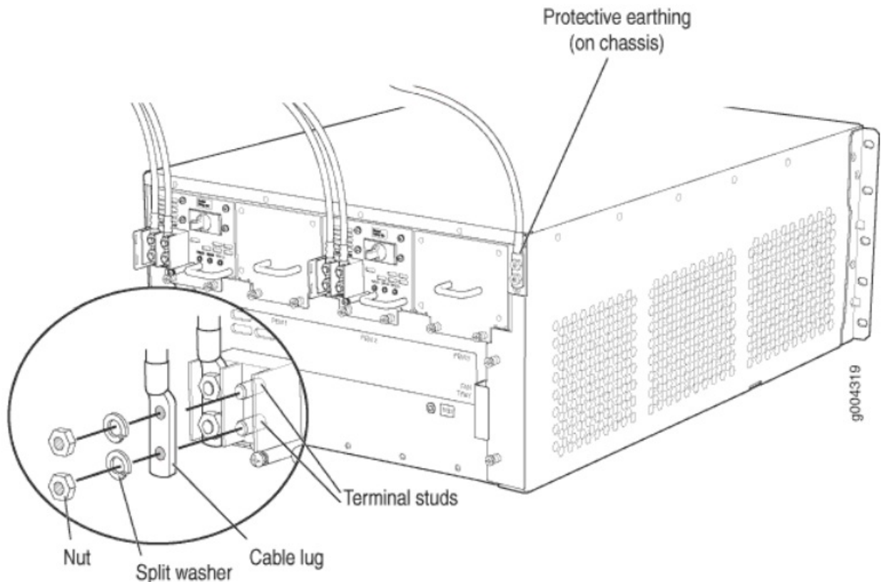
Figure 11: Connect Power Cables
