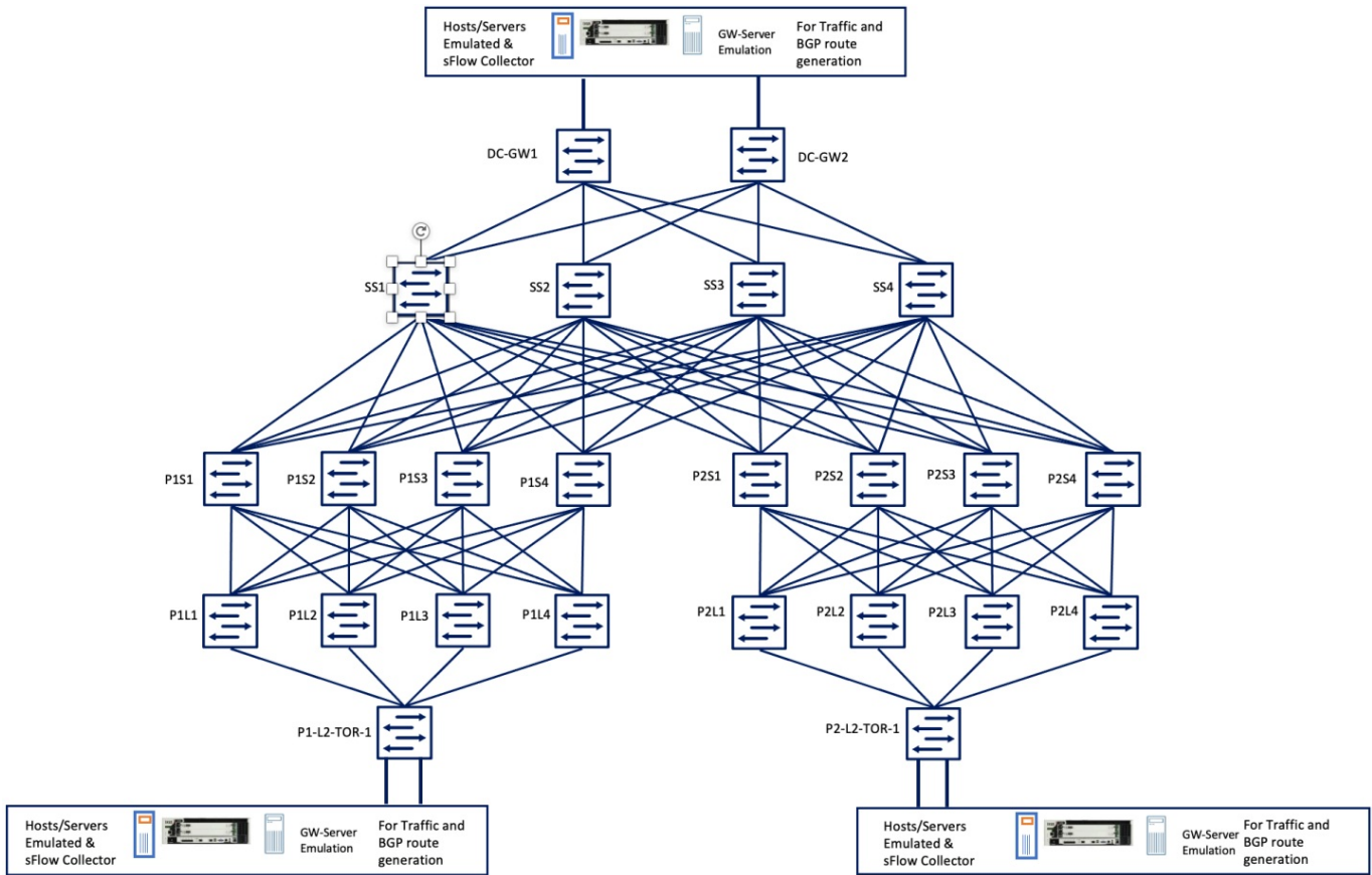
Figure 1: IP Fabric Topology with EBGp Fabric Protocol, with Every Layer in Different AS Routed Fabric with Super Spine Architecture
