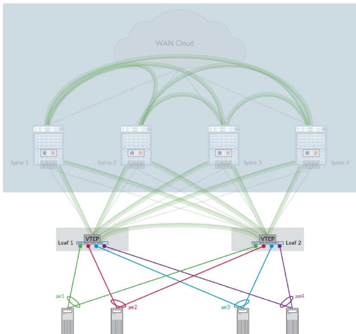
Figure 2: EVPN LAGs in a CRB Architecture
