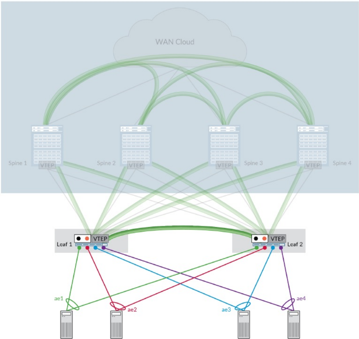
Figure 3: EVPN LAGs in ERB Architecture
