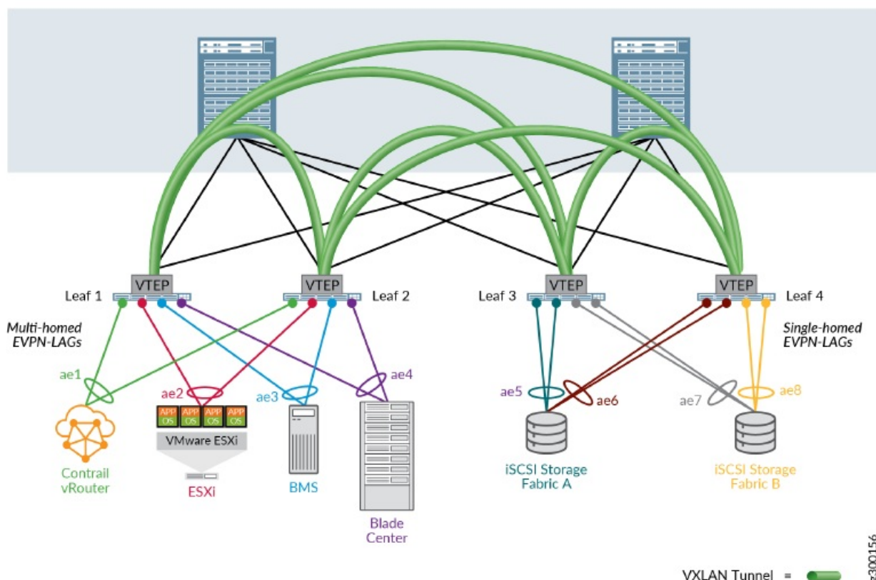
Figure 1: Data Center Example Topology with EVPN LAGs
