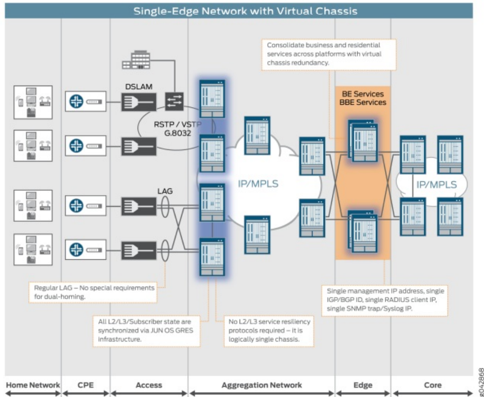
Figure 8: Single-Edge Architecture
