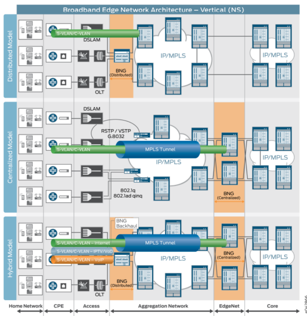
Figure 5: Broadband Edge Network Architectural Models
