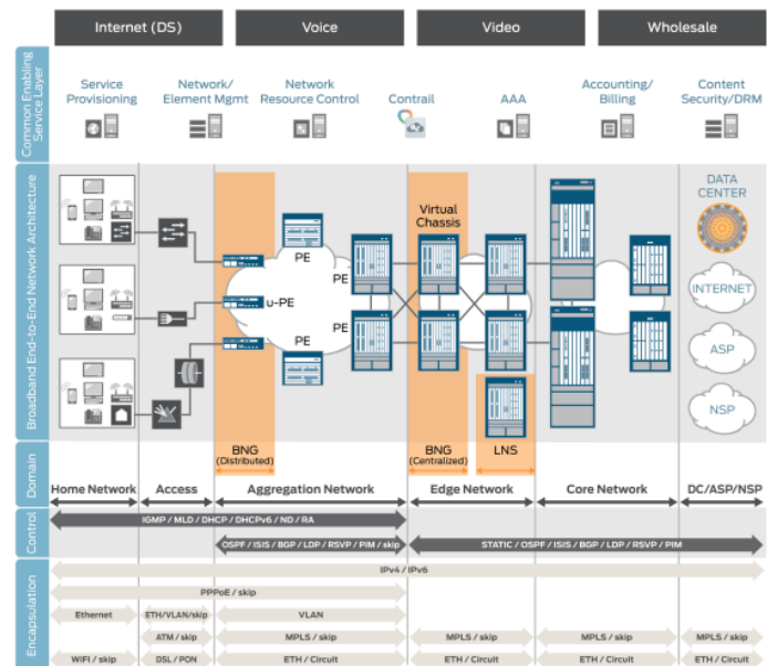
Figure 2: The Broadband Edge Architecture
