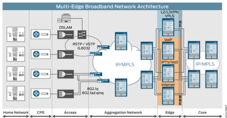
Figure 7: Multi-Edge Network Architecture
