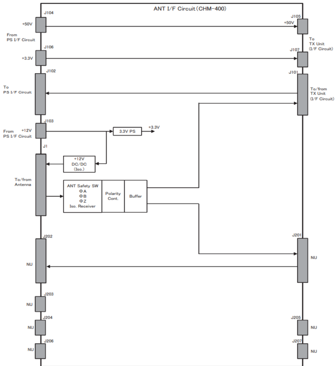
Fig. 3.1.2-1 ANT I/F Circuit Block Diagram
