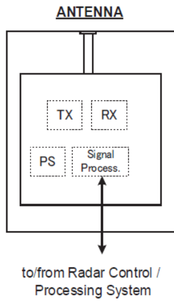
Fig.2 (1) NTG-560 Configuration Diagram
