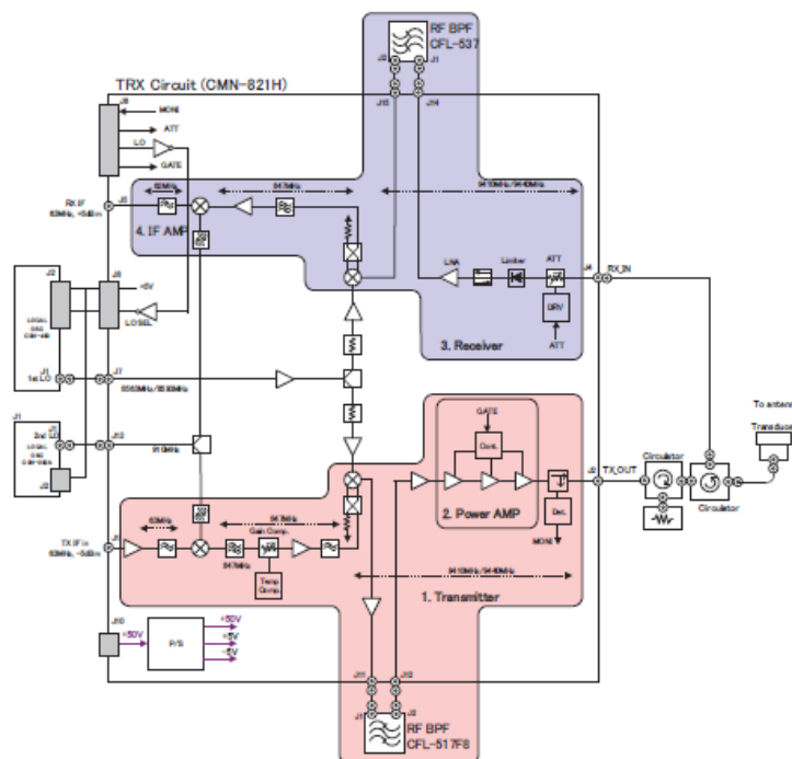
Fig. 3.1.1-1 TRX Unit Block Diagram
