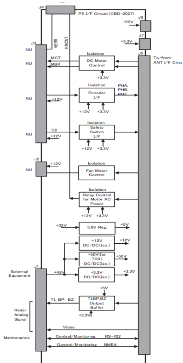
Fig. 3.3-1 PS I/F circuit Block Diagram
