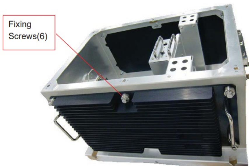
Fig. 5-1 NTG-560 X-band Solid State Transmitter-Receiver Internal View
