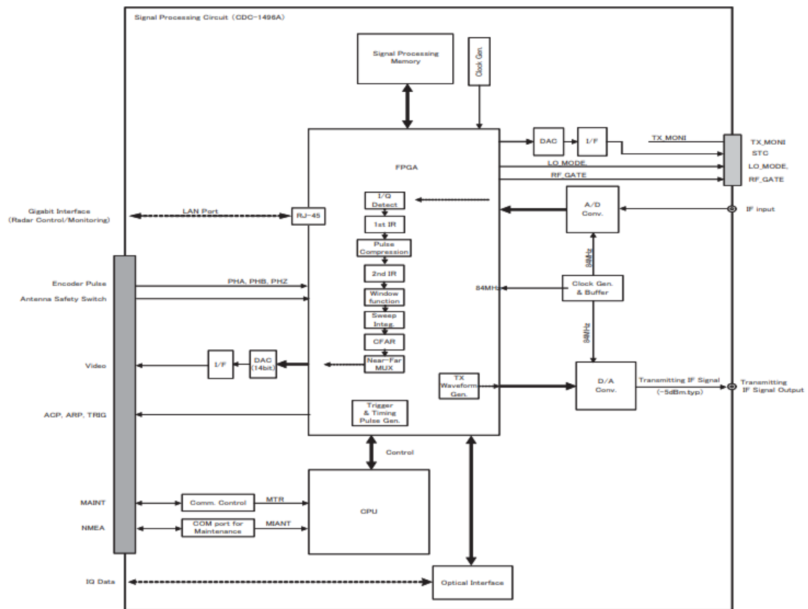
Fig. 3.1-1 Signal Processing Circuit Block Diagram
