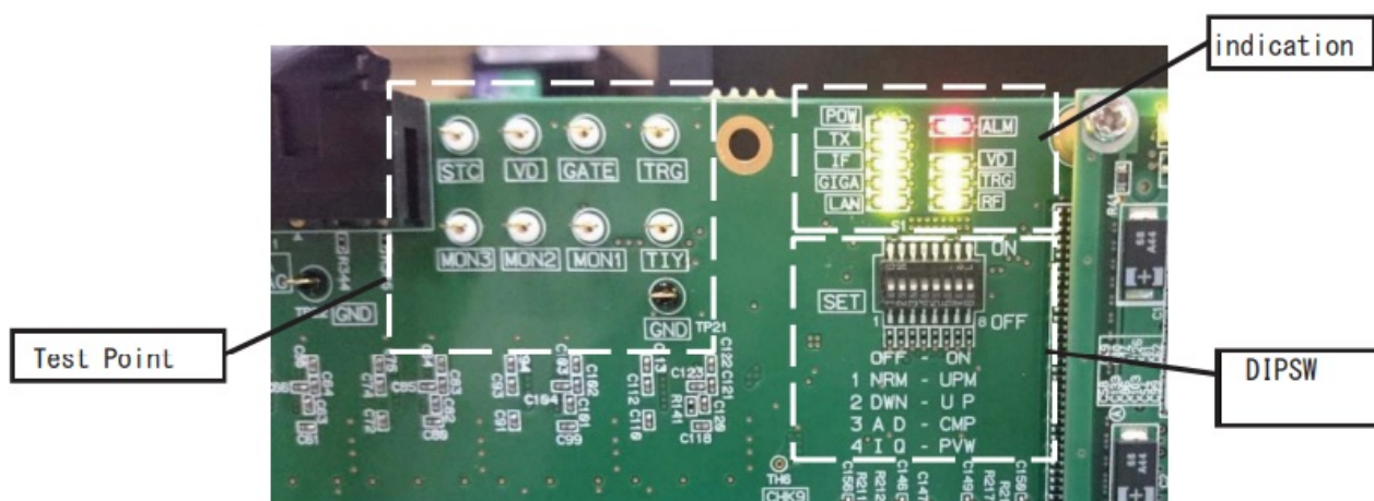
Fig. 4-1 S/P Circuit LED Location
