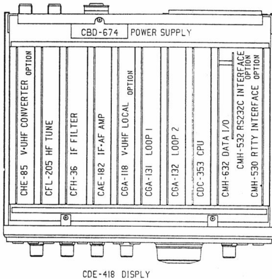
Fig. 9-3 Location of Units
