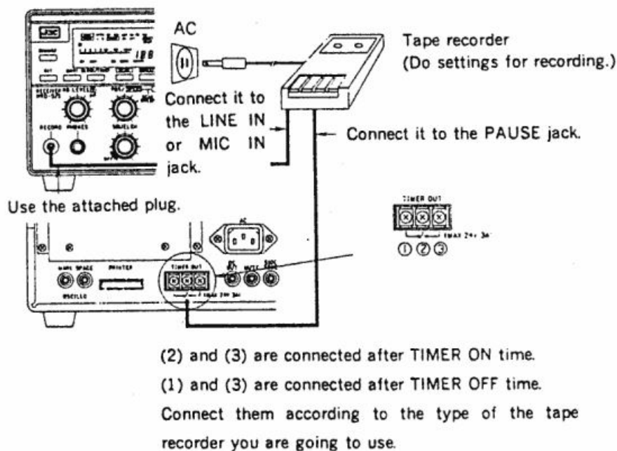
Fig. 5-2 Connection of Tape Recorder
