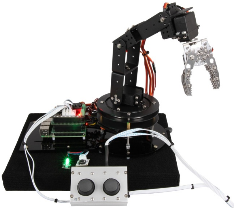
Image 1: Robot02 with optional accessories
